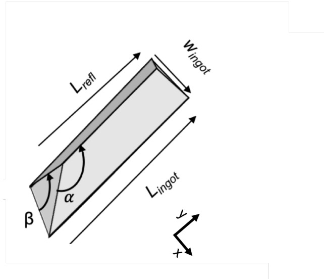
Figure 1. Schematic representation of the ingot solid shape and the parameters used to describe its geometry. The reference axes used to calculate the slopes are shown in the corner. Note that the simulation tool described in this work accepts the projection of ingot length on the FP, L_{in,FP} , instead of its total length L_{ingot} , as indicated in Table 1. L_{refl} is the minimum length of the reflective face.
