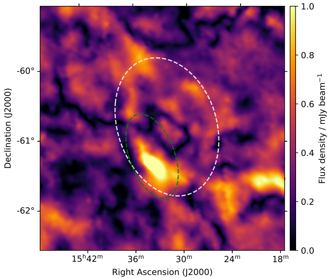
Fig. A.1. Total linear polarization of 3^{\circ}5 \times 3^{\circ}5 deg of the region surrounding G321.3-3.9 estimated from Stokes Q and U images of S-PASS. The white dashed line highlights the remnant shell, and the green dashed line corresponds to the polarized part of the shell we examined.
