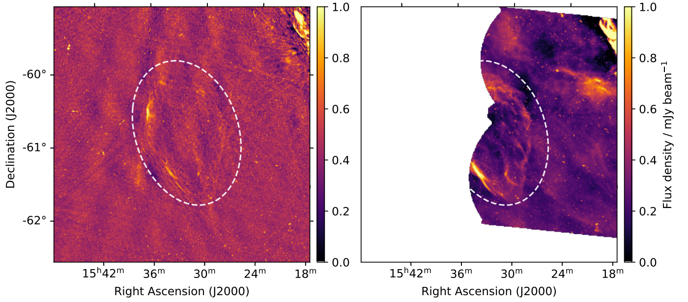
Fig. B.1. 3.5 \times 3.5 deg of the region surrounding G321.3–3.9 as seen at \sim 888 MHz by RACS in the left panel and at 944 MHz by EMU in the right panel.
