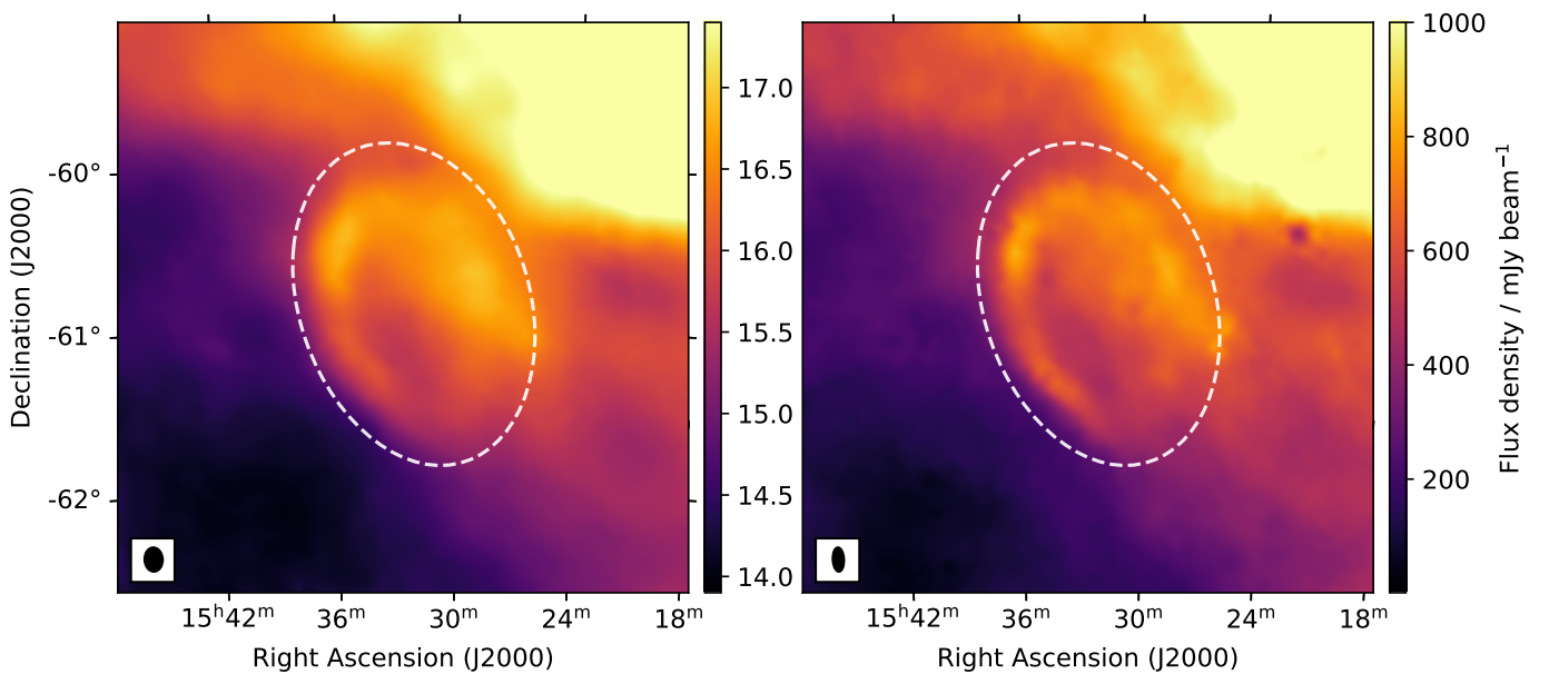
Fig. 2. 3.5 \times 3.5 of the region surrounding G321.3–3.9 as seen at 1.4 GHz by CHIPASS (left panel) and at 2.3 GHz by S-PASS (right panel). The panels show the region after the conversion from K to \text{Jy beam}^{-1} and the subtraction of point sources. The dashed line highlights the area within which the SNR is located.
