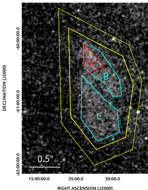
Fig. 4. eRASS:4 smoothed image of G321.3–3.9 in the 0.5 – 2.4 keV energy range with regions used for the eROSITA X-ray spectral analysis. The main source region is the solid yellow polygon surrounding the SNR. The point sources subtracted from the field are highlighted by a green circle with a red line in the center. The background region is the area between that polygon and the bigger dotted polygon.
