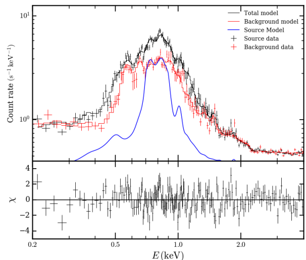
Fig. 5. X-ray spectrum of G321.3–3.9 obtained with eROSITA. The fit model is TBabs*vapec .
