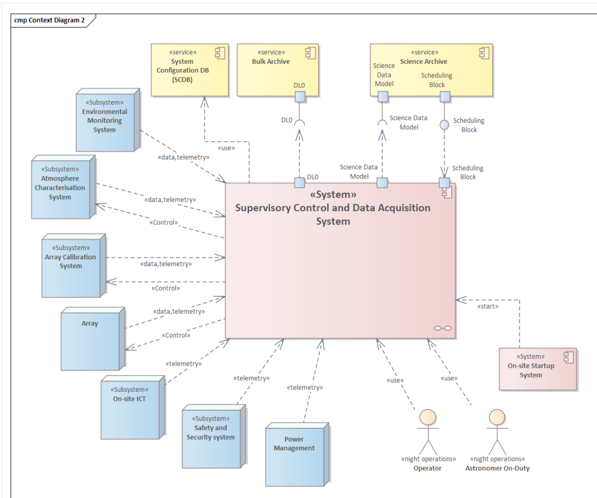
Figure 4: SCADA context diagram.
