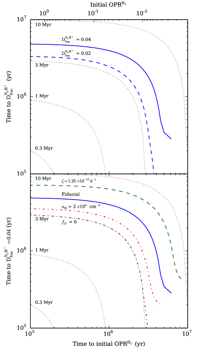
Figure 7. Time to reach the observed deuterium fraction ( \text{D}_{\text{frac}}^{\text{N}_2\text{H}^+} = 0.04 ) from a given initial ortho-to-para ratio of H 2 (shown on the top axis) versus the time to reach this initial ortho-to-para ratio if starting from statistical equilibrium ratio of 3. The solid blue line shows this result for the fiducial model parameters, e.g. of density, temperature, depletion factor, cosmic ray ionization rate. Grey dotted lines show contours of the sum of the deuteration time-scale and ortho-to-para ratio decay time-scale to equal 0.3, 1, 3, 10 Myr, as labeled. The dashed blue line (upper panel) shows the time to reach \text{D}_{\text{frac}}^{\text{N}_2\text{H}^+} = 0.02 for the fiducial model. The dashed and dot-dashed lines (lower panel) show the effect of varying several of the model parameters, as labeled.
