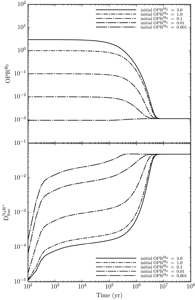
Figure 6. Time evolution of the \text{OPR}^{\text{H}_2} (upper panel) and \text{D}_{\text{frac}}^{\text{N}_2\text{H}^+} (lower panel) under different assumptions of the initial \text{OPR}^{\text{H}_2} , for n_{\text{H}} = 10^4 \text{ cm}^{-3} , f_{\text{D}} = 3 , T_{\text{kin}} = 15 \text{ K} , and A_{\text{v}} = 20 \text{ mag} . We explore \text{OPR}^{\text{H}_2} from 3 down to 0.001.
