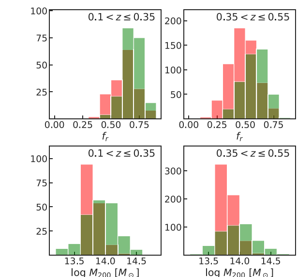
Figure 10. Distribution in fraction of red galaxies ( f_r ) and mass (from AMICO) in two-redshift bins for the matched (green) and unmatched (red) clusters from the KiDS-AMICO versus redMaPPer catalogues. A cut on mass, \log M_{200} > 13.5 M_{\odot} , was applied to unmatched clusters.
