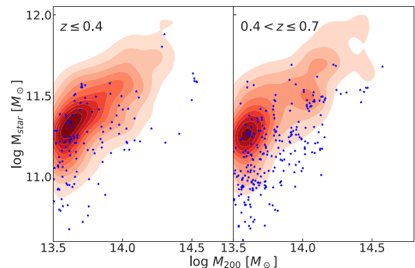
Figure 16. BCG stellar masses versus cluster masses in the Illustris TNG300-1 sample: red contours display the distribution for red BCGs, values for blue BCGs are plotted as blue stars.
