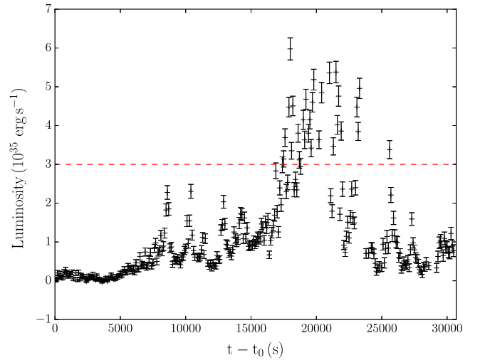
Figure 8. The XMM-Newton light curve shown in Fig. 4 with count rate converted into luminosity using an absorbed power law with photon index \Gamma = 1.9 , absorbing column density, n_H = 5 \times 10^{23} \text{ cm}^{-2} and a source distance of 2.1 \pm 0.1 \text{ kpc} . The red dashed line corresponds to the critical luminosity for transition between the radiatively cooled to Compton-cooled regimes in Shakura et al. (2013).
