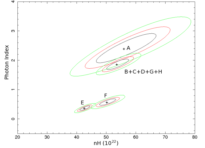
Figure 7. Confidence contours for the best-fitting spectral parameters to regions A, B+C+D+G+H, E and F using an absorbed power-law model [ \text{cons} * \text{phabs} * \text{cflux}(\text{powerlaw}) ] with the 68 per cent, 90 per cent and 99 per cent statistical confidence regions shown.
