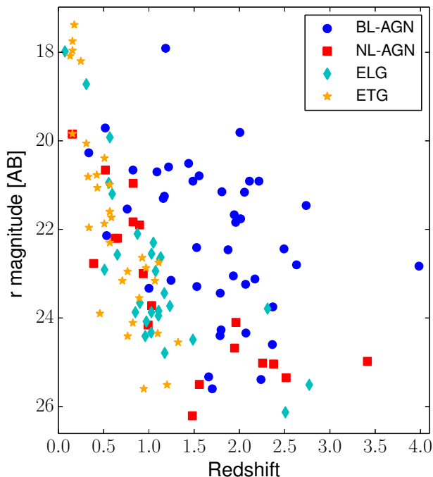
Fig. 4. Total AB magnitude in the r band from Nanni et al. (2020) as a function of spectroscopic redshift for 122 Chandra J1030 sources with z_{\text{spec}} : we do not include in this plot the z=6.3 QSO SDSSJ1030+0525, which is not detected in the r -band. BL-AGNs are plotted as blue circles, NL-AGN as red squares, ELGs as cyan diamonds, and ETGs as orange stars.
