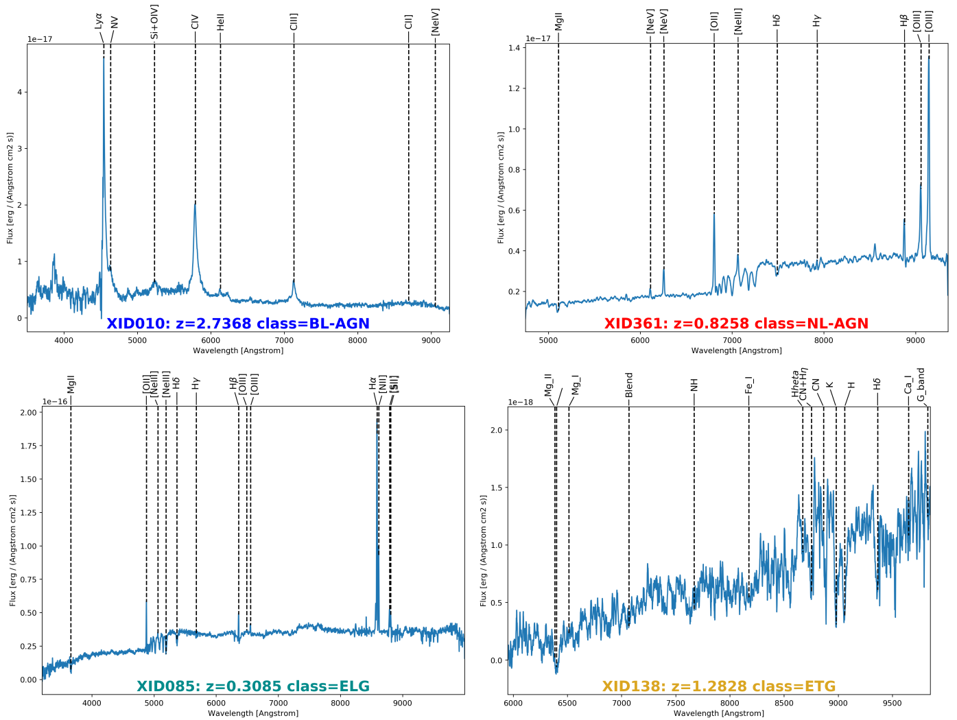
Fig. 3. Example of MODS spectra of four Chandra J1030 optical counterparts: all the spectra have been obtained with the LBT strategic program. From the top left, moving clockwise: XID-10 (broad-line AGN); XID-361 (narrow-line AGN); XID-138 (early type galaxy); XID-85 (emission-line galaxy).
