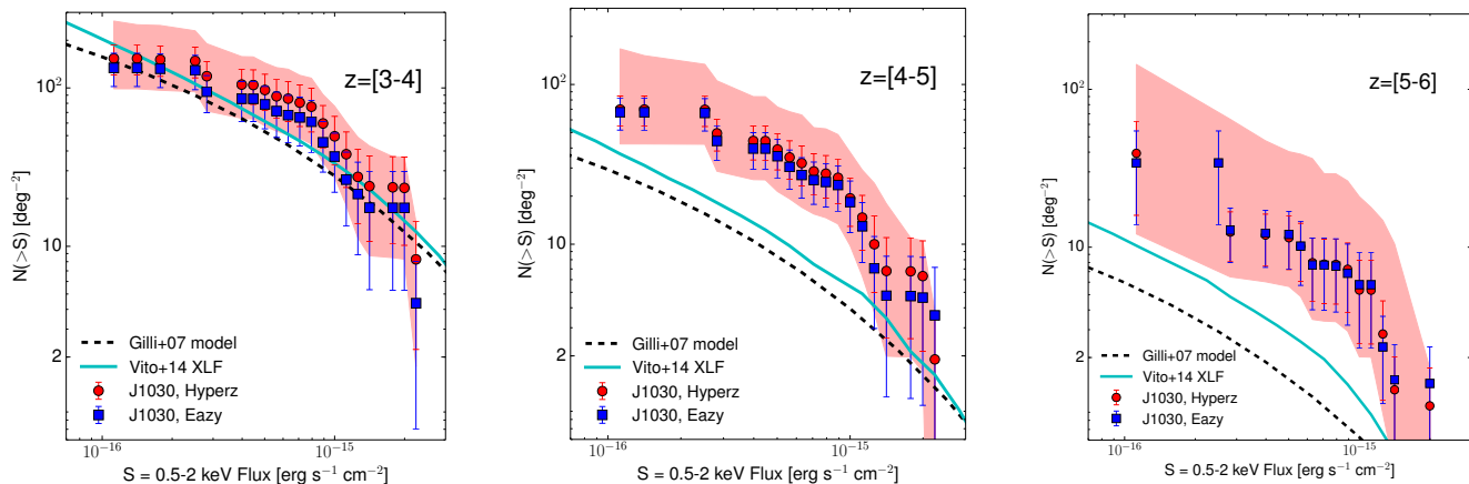
Fig. 15. Chandra J1030 0.5–2 keV number counts computed using the Hyperz photometric redshifts (red circles in the redshift bins z=[3-4] (left), z=[4-5] (center), and z=[5-6] (right)). The upper boundary of the shaded area is computed including the “low-reliability” sources defined in the text and two objects lacking a counterpart. The lower boundary is computed assuming a conservative PDZ shape (see the text for more details). The number counts derived using the EAZY photometric redshifts (blue squares) are also plotted for comparison. The number counts in the same redshift ranges derived using the Gilli et al. (2007) AGN population synthesis model (black dashed line) and the Vito et al. (2014) XLF (cyan solid line) are also shown for comparison.
