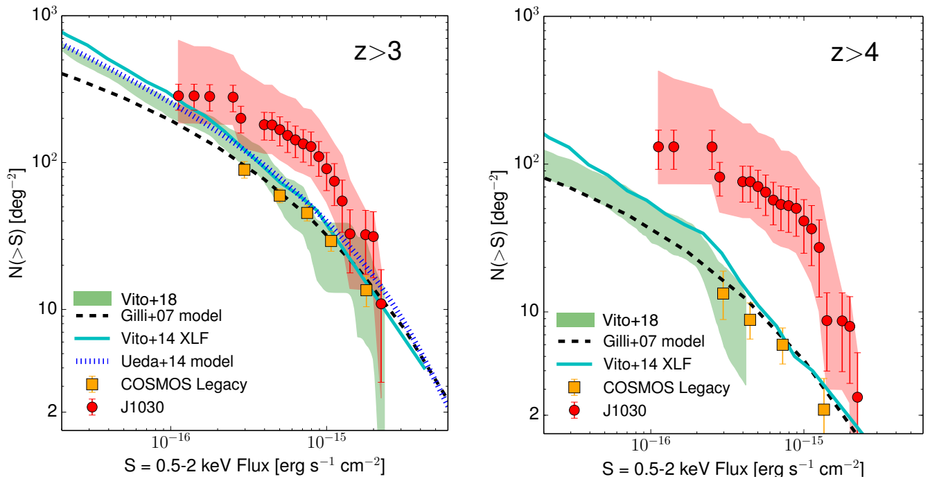
Fig. 14. z > 3 (left) and z > 4 (right) number counts for Chandra J1030 (red circles): the error bars are the Poissonian uncertainties. The upper boundary of the shaded area is obtained including in the computation 21 “low-reliability” sources, which are those objects with only a K -band and/or an IRAC-band detection, as well as two objects with no counterpart. The lower boundary is computed assuming a conservative PDZ shape (see the text for more details). The number counts obtained in the same redshift range in the Chandra COSMOS-Legacy survey (orange squares, Marchesi et al. 2016b) and in the CDF-S and CDF-N surveys (green area Vito et al. 2018) are also shown for comparison, together with the predictions from the Vito et al. (2014, cyan solid line) and Ueda et al. (2014, blue dotted line) X-ray luminosity functions, and those of the Gilli et al. (2007) AGN population synthesis model.
