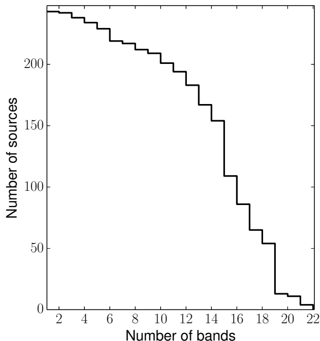
Fig. 5. Cumulative distribution function of the number of bands in which a source has been detected.
