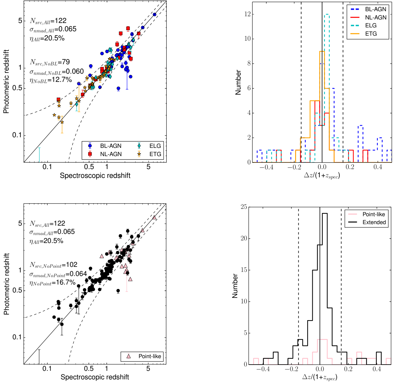
Fig. 7. Left: Photometric redshift as a function of the spectroscopic one for the 122 J1030 sources with an available spectroscopic redshift. The black solid line marks the z_{\text{spec}}=z_{\text{phot}} relation, while the dashed lines contain the z_{\text{phot}}=z_{\text{spec}}\pm 0.15(1+z_{\text{spec}}) region. Sources within this region are deemed to have a reliable photometric redshift. In the two panels, we highlight different classes of sources which are more likely to have a large fraction of outliers: spectroscopically classified BL-AGN (blue circles, top); morphologically-classified point-like sources (pink triangles, bottom). Right: Distribution of \Delta z/(1+z_{\text{spec}}) for the sources reported in the left panel. The color code is the same of the two figures on the left.
