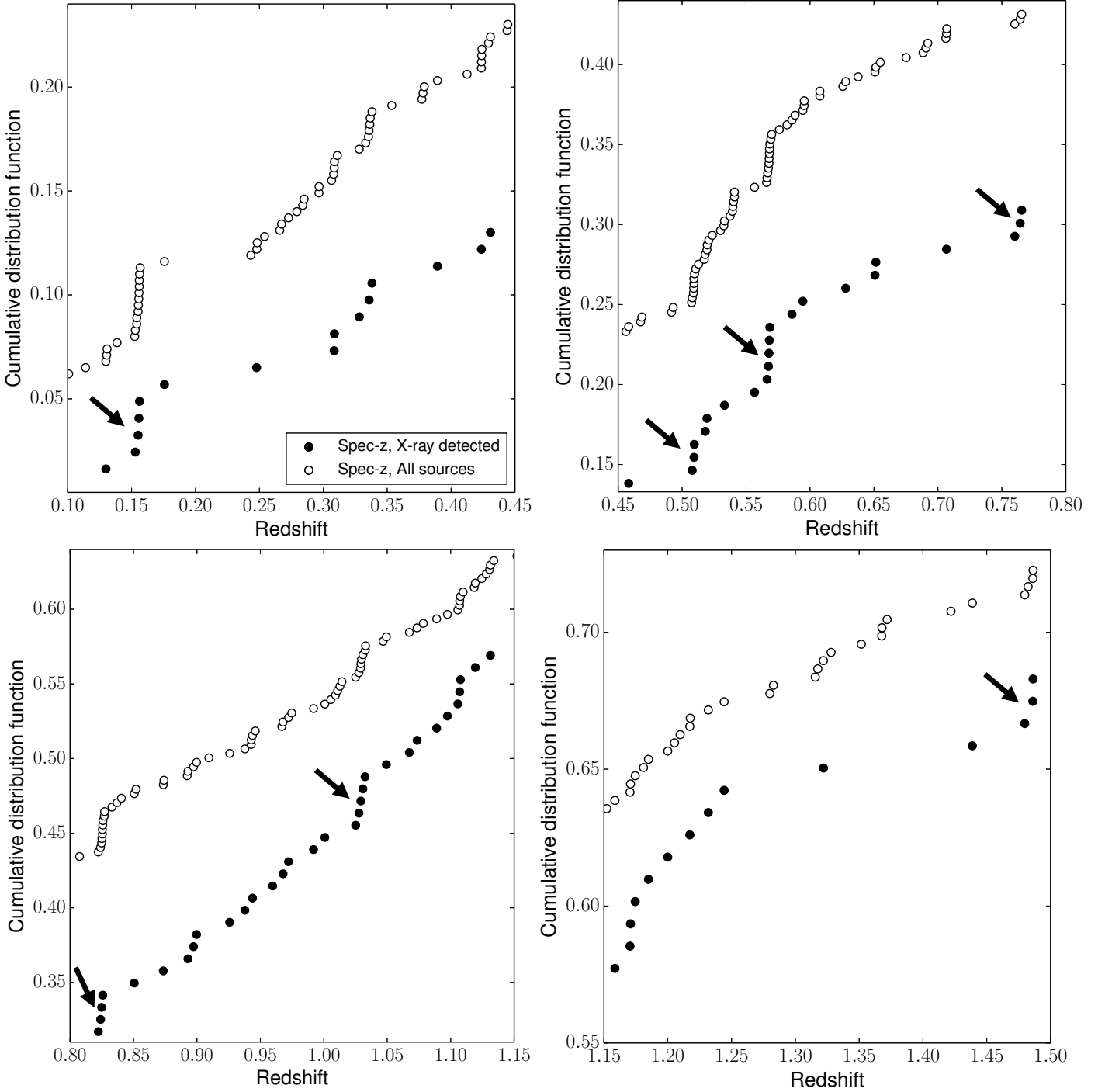
Fig. 12. Cumulative distribution function for the Chandra J1030 sources with a spectroscopic redshift (full markers), and for all the J1030 sources with a spectroscopic redshift, including the non-X-ray detected ones (empty markers). The overall CDF distribution is shifted by 0.05 for visualization purposes. The structures identified within the Chandra J1030 population are marked with arrows: as it can be seen, the X-ray sources effectively track the overall population.
