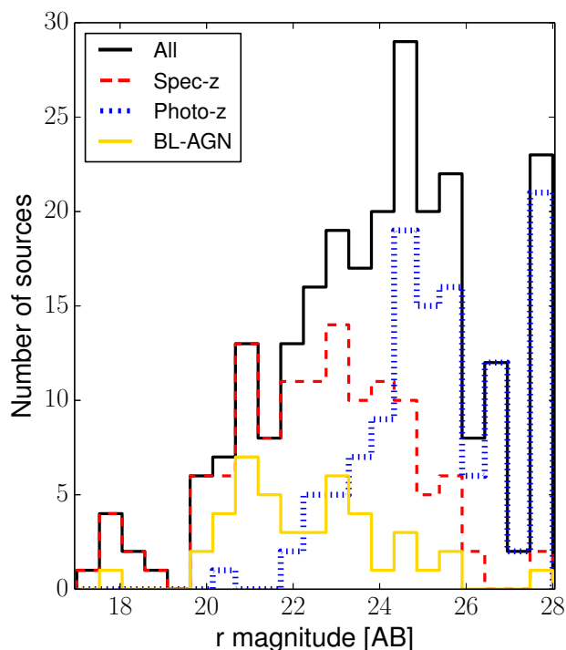
Fig. 8. AB magnitude in the r band of all the 243 extragalactic sources in the Chandra J1030 sample having an optical/nIR counterpart (solid black line), the 123 sources with spectroscopic redshift (dashed red line), the 120 sources with only photometric redshift (dotted blue line) and the 43 broad-line AGNs (solid yellow line). We assign to the 24 sources with no r -band detection a magnitude r_{\text{AB}} = 27.5 , which is their upper limit. The BL-AGN with an r -band upper limit at r_{\text{AB}} = 27.5 is the z = 6.3 QSO SDSSJ1030+0525.
