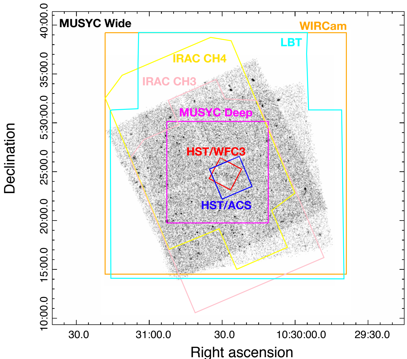
Fig. 1. Smoothed 0.5–7 keV Chandra ACIS-I image of the SDSS J1030+0524 field. The regions covered by the photometric catalogs used in this work are also shown in different colors. The whole J1030 field has also been imaged in the mid-infrared IRAC channels 1 and 2.
