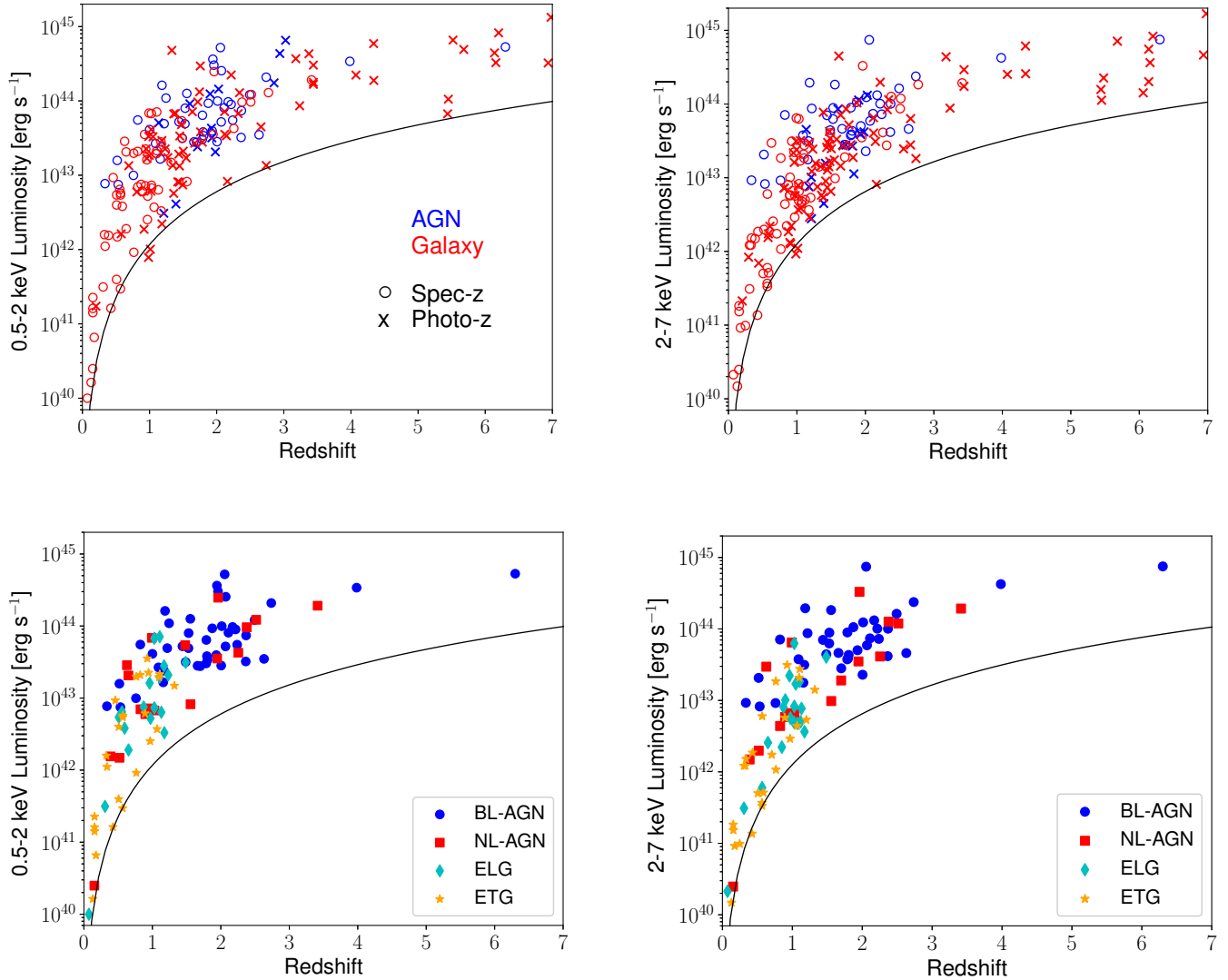
Fig. 11. Top: Intrinsic, absorption-corrected luminosity in the 0.5–2 keV (left) and 2–7 keV (right) band as a function of redshift. Sources with a spectroscopic redshift are plotted with circles, while sources with only a photometric redshift are plotted with crosses. Sources with a BL– or NL-AGN spectrum or with a SED best-fitted with an AGN template are plotted in blue, while sources with a ETG or ELG spectrum, or with a SED best-fitted with a galaxy template are plotted in red. We also plot as a black solid line the luminosity corresponding to the flux at which 10% of the field is covered. Bottom: same as above, but for the spectroscopic subsample alone. BL-AGNs are plotted as blue circles, NL-AGNs as red squares, emission line galaxies as cyan diamonds, and early type galaxies as orange stars.
