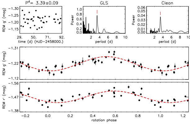
Fig. 2. Same as in Fig. 1 but for the REM g' -filter. In the bottom panel, we plot also the r' color curve phased with the rotation period.
