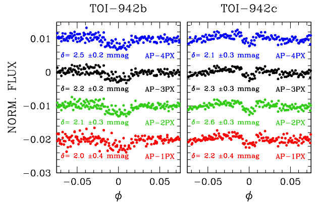
Fig. 10. Phased light curves for TOI-942 b (left panel) and TOI-942 c (right panel) obtained with different apertures marked with different colors.
