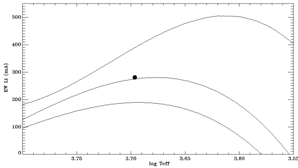
Fig. 7. Lithium EW vs effective temperature for TOI-942 and sequences of ScoCen, IC 2602 and Pleiades from Pecaut & Mamajek (2016) .
