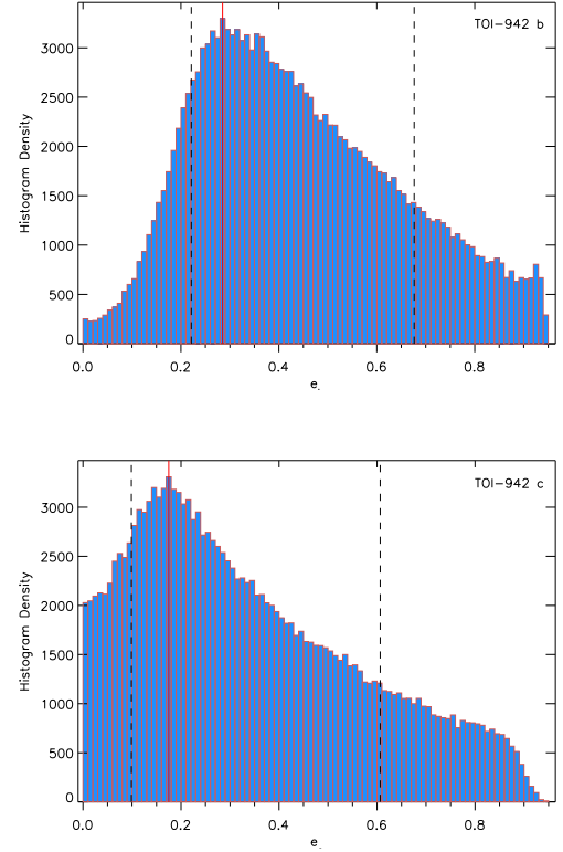
Fig. 14. The posterior distribution for the eccentricity of TOI-942 b (upper panel) and TOI-942 c (lower panel). The vertical red line indicates the maximum value of the distribution, while the dashed lines indicate the 16-th and 84-th percentiles.
