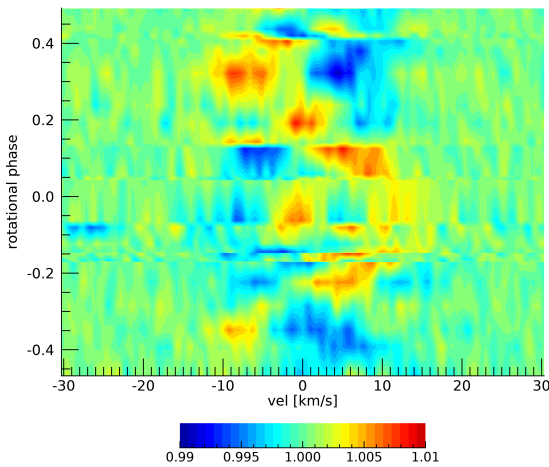
Fig. 6. Contour map of the CCF residuals of TOI-942 versus radial velocity and rotational phase. The color bar indicates relative CCF amplitude with respect to the mean CCF.
