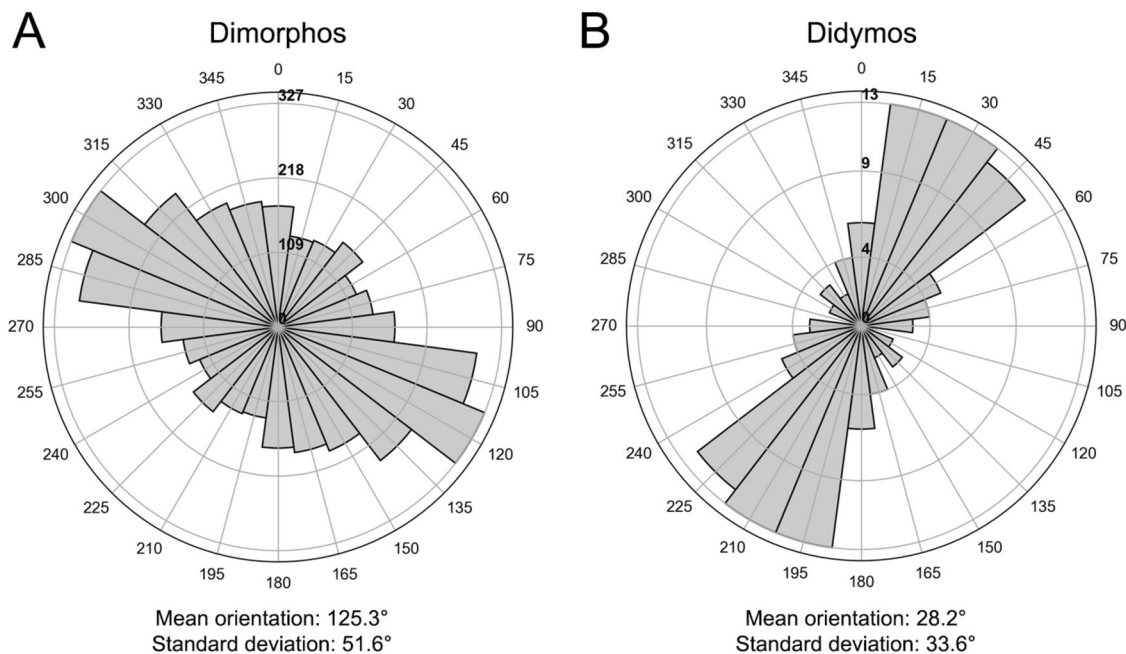
Fig. 8 | Dimorphos and Didymos boulder orientations. Rose diagrams of Dimorphos ( A ) boulders \geq 1 m and of Didymos ( B ) boulders \geq 16.5 m with an apparent axial ratio < 0.9 . The corresponding mean orientation and standard deviation are also indicated. We recall that Dimorphos is tidally locked with respect
