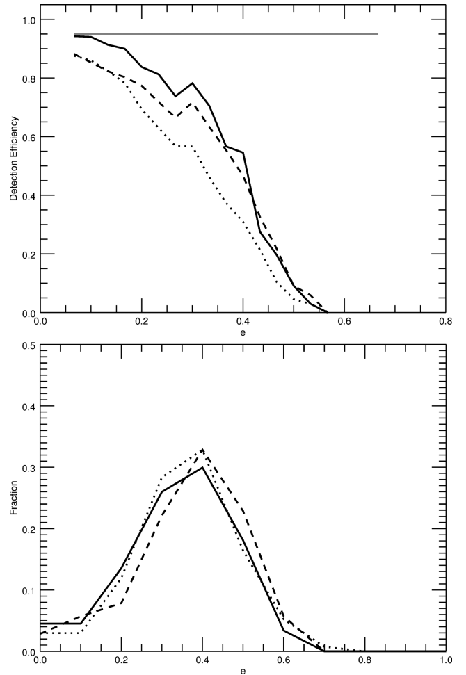
Figure 7. Top: detection efficiency above the 10^{-3} FAP threshold as function of eccentricity. The solid black line is for GLS, the dashed black line for BGLS and the dotted black line for FREDEC. The grey solid line indicates the 95 per cent level. Bottom: histogram of the fraction of significant periods identified in the residuals as function of eccentricity. Line coding is the same as in the upper panel.
