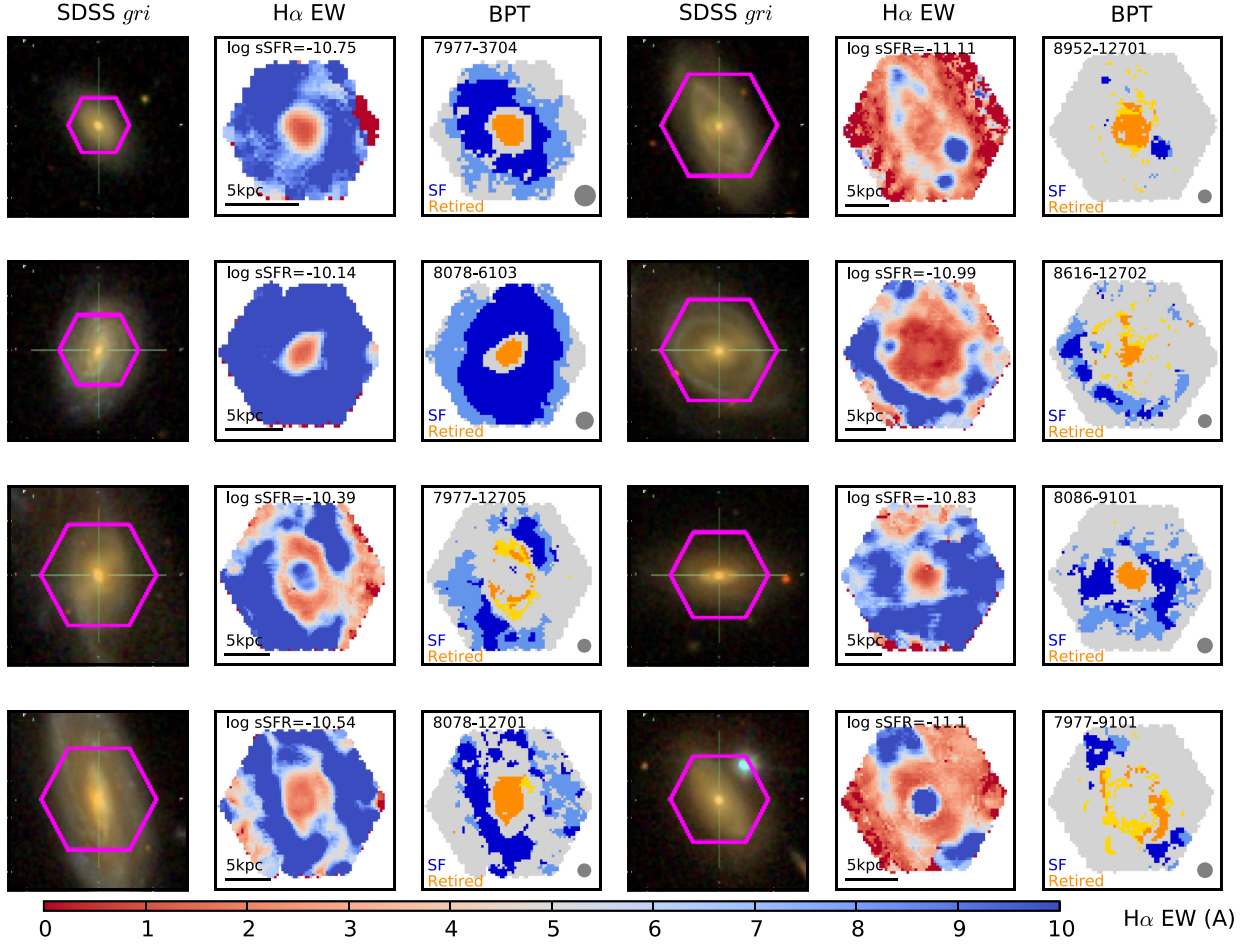
Figure 2. The eight galaxies selected from the ALMaQUEST sample which have sufficient ( >20 ) spaxels to investigate the rMGMS for star-forming and retired populations of spaxels. The first and fourth columns show the SDSS images with the hexagonal MaNGA footprint shown in magenta; the second and fifth columns show the H\alpha EW maps (see colour bar along the lower edge of the figure); the third and sixth columns show the maps of spaxel classifications. Retired spaxels are shown in orange and star-forming spaxels in blue, with paler shades of each colour indicating a CO non-detection in CO. Spaxels that do not fall into either of these two classes are shown in grey. The filled grey circle indicates the median FWHM (full width at half maximum) of 2.5 arcsec (Law et al. 2015).
