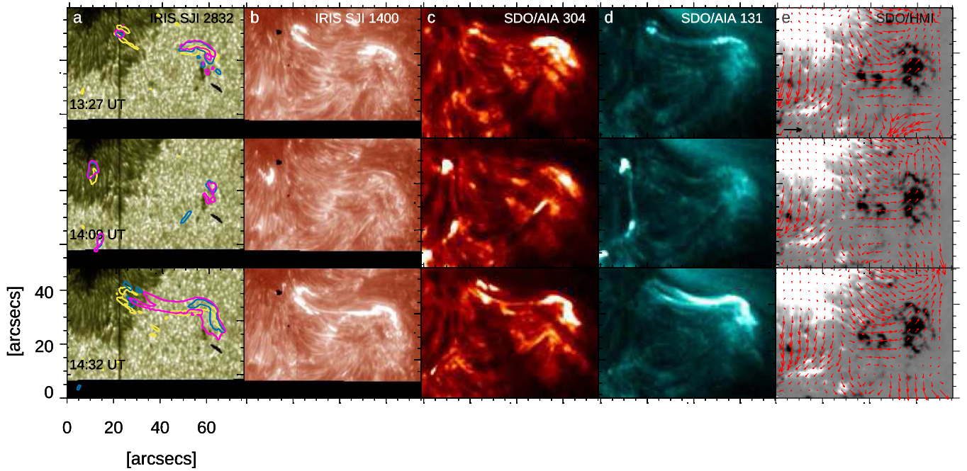
Figure 6. Examples of the SDO and IRIS data analyzed in our study, relevant to the ROI. From left to right: (a) IRIS I2832, (b) IRIS I1400, (c) SDO /AIA 304, and (d) SDO A131 filtergrams. Column (e) displays the maps of the LOS magnetic field from SDO /HMI data with the horizontal velocity field derived from the same observations overplotted. The light curves in Figure 5 were computed over the FoV shown in these panels. The colored contours overplotted on the IRIS I2832 data represent the footpoints and regions of maximum brightening in the IRIS I1400 (green), SDO /AIA A131 (red), and A304 (blue) measurements, respectively. The black arrow in panel (e) represents a horizontal velocity of 1 \text{ km s}^{-1} .
