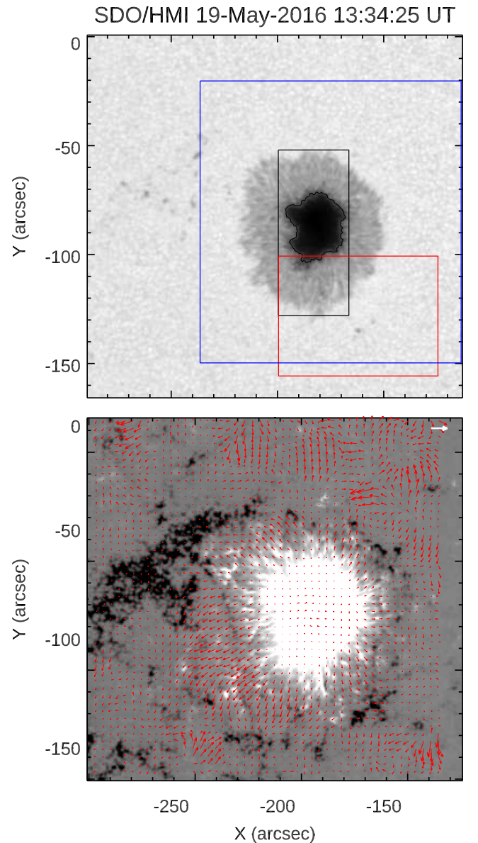
Figure 1. Subarray extracted from the full-disk continuum filtergram (top panel) and LOS magnetogram (bottom panel) taken by SDO /HMI on May 19 at 13:34 UT and centered on the studied AR. Values of the LOS component of the magnetic field are saturated at \pm 500 G. The black and blue boxes indicate the FoV of the IBIS and IRIS observations analyzed in our study, respectively, while the red box shows the ROI where the studied brightening events occur. Here and in the following figures, solar north is to the top, and west is to the right. The horizontal velocity estimated with FLCT is overplotted on the LOS magnetogram. The white reference arrow indicates a horizontal velocity of plasma of 1 \text{ km s}^{-1} . See Sections 2 and 3 for more details.
