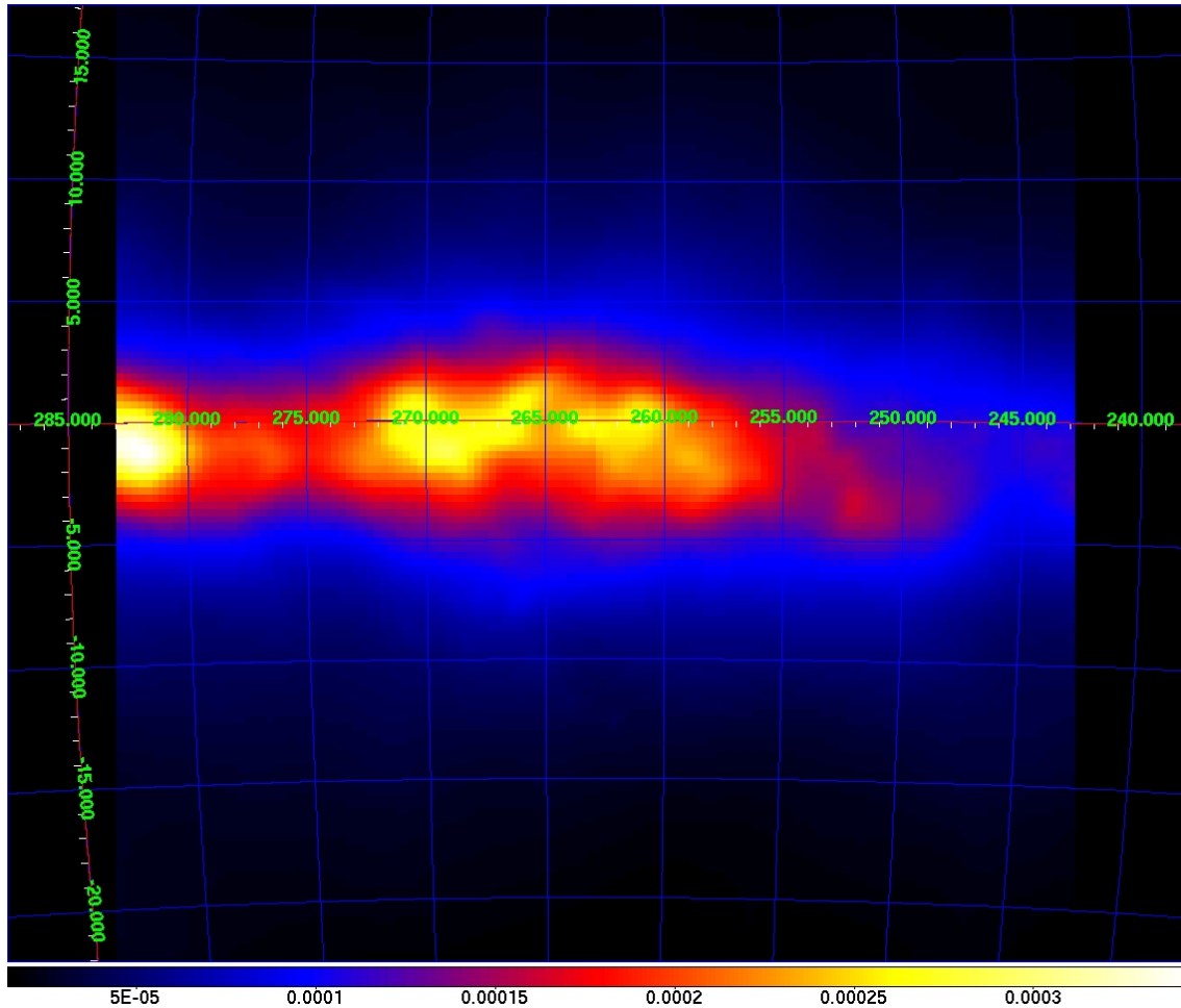
Figure 4: DS9 image of the diffuse emission map produced by AG_gasmapgen with the listed parameter file.
