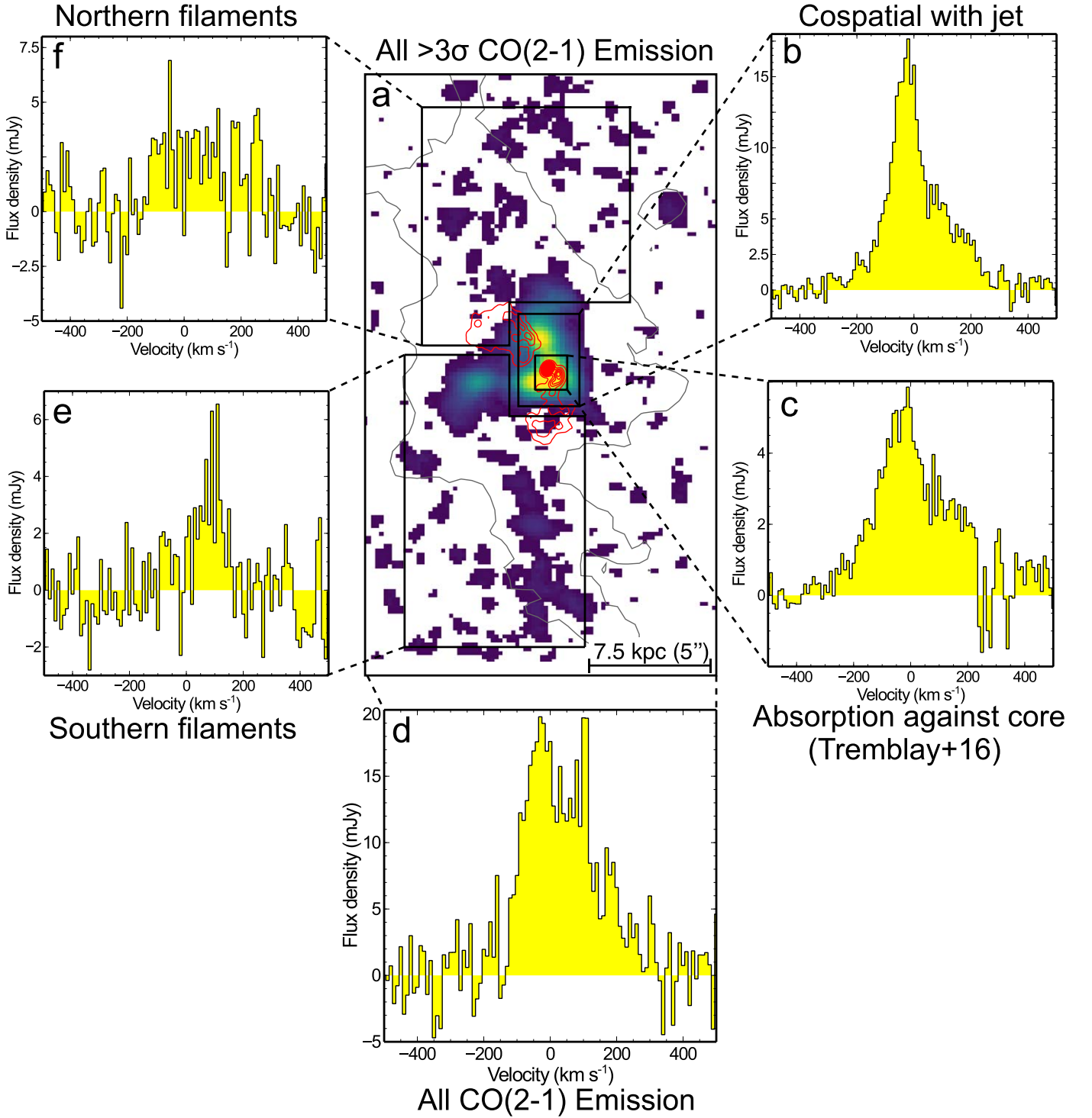
Figure 5. An overview of the morphological and spectral characteristics of the ALMA CO(2-1) observation we discuss at length in this paper. The central panel (a) shows a clipped moment zero (flux) image of all \geq 3\sigma CO(2-1) emission in the A2597 BCG. The various clumps seen likely represent \geq 3\sigma peaks of a smoother, fainter distribution of gas below the sensitivity threshold (although some clumps may indeed be discrete). For reference, the outer contour of the H \alpha nebula is shown with a solid gray contour. Various apertures are shown in black polygons, indicating the (rough) spectral extraction regions for the CO(2-1) line profiles shown in the surrounding panels. All data are binned to 10 km s -1 channels. (b) The CO(2-1) line profile from a region cospatial with the \sim 10 kpc scale CSS radio source (red contours on panel (a)). (c) An extraction from the nucleus of the galaxy, cospatial with the millimeter and radio core, as well as the stellar isophotal centroid. The deep absorption features are discussed in Section 3.1 and Tremblay et al. (2016). (d) All detected emission across the entire nebula. It is from this spectrum that we estimate the total gas mass in Section 3.3. Panels (e) and (f) show the spectra extracted from what we call the southern and northern filaments, respectively.
