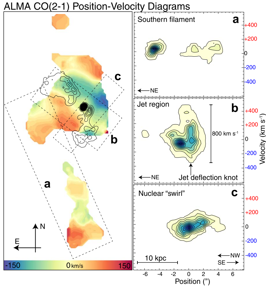
Figure 7. Position–velocity (PV) diagrams extracted from the three regions of the molecular nebula. The lefthand panel shows the moment one velocity map from Figure 6, with three PV extraction apertures overlaid. The righthand panels show the PV diagrams extracted from these apertures. Arrows are used to show the cardinal orientation of each aperture’s long axis (the slit orientation for panel (c) is roughly perpendicular to that for panels (a) and (b), and so the relative orientations are admittedly confusing at first glance). Note that while the length of the extraction aperture varied, all diagrams are shown on the same spatial scale in the righthand panels, enabling cross-comparison. Panel (a) shows that the southern filament has a narrow velocity width across its entire length, and no coherent velocity gradient. Panel (b) reveals the broadest velocity distribution of molecular gas in the entire nebula and includes the region in which the 8.4 GHz radio source bends in position angle, likely because of deflection. Panel (c) shows the rotation of molecular gas about the nucleus. All emission shown is \geq 3\sigma .
