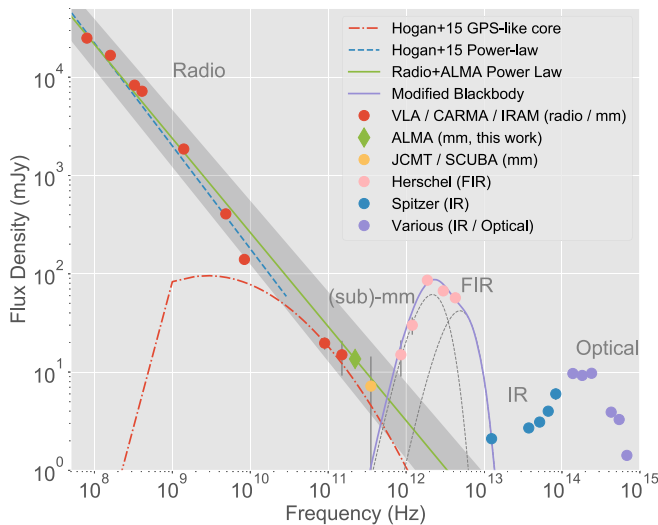
Figure 3. Radio-through-optical SED for Abell 2597, including the new ALMA millimeter continuum point. Dashed and solid lines show various fits to components of the spectrum including a one- and two-component fit to the radio and ALMA data (Hogan et al. 2015a, 2015b), as well as a modified blackbody fit to the far-infrared Herschel data (Mittal et al. 2011, 2012). Observation details (including dates) and references for all photometric points are given in Table 1. Error bars are shown on the plot, though in many cases they remain invisible because they are smaller than the data point. The gray shaded region shows the error on the single power-law fit to both the radio and ALMA continuum data. These fits are discussed in Section 3.1.
