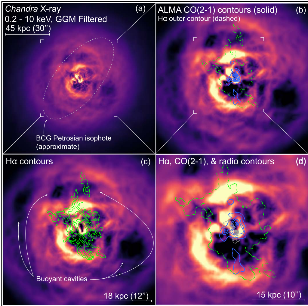
Figure 18. A new, deeper look at the X-ray cool core cospatial with the A2597 BCG. (a) 626 ks Chandra X-ray observation of 0.2–10 keV emission in the innermost \sim 250 \times 250 kpc 2 of the cluster. The X-ray data have been convolved with a GGM filter (e.g., Sanders et al. 2016a) to better show ripples and cavities. The optical Petrosian radius of the BCG’s stellar component is (roughly) marked by the gray dashed ellipse. Brackets indicate the relative FoVs shown in the surrounding panels. Panels (b), (c), and (d) show the same data, slightly zoomed in, with MUSE H \alpha , ALMA CO(2–1), and 8.4 GHz radio contours overlaid in green, blue, and gray, respectively. Moving inward, the ALMA contours in panel (d) show emission that is 3\sigma , 5\sigma , 10\sigma , and 20\sigma over the background rms noise level. With the caveat that projection effects complicate interpretation, the H \alpha nebula shows strong circumstantial evidence that at least some of the filaments are draped around the edges of the buoyant X-ray cavities marked by arrows.
