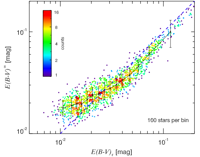
Fig. G.1. Total reddening observed in the optical, E(B - V)^\infty , as a function of E(B - V)_\tau , the dust optical depth at 353 GHz converted to a reddening, for the 1505 selected stars (Sect. 6.3). Each bin of the running mean contains the same number of lines of sight. Error bars represent the standard deviation in each bin. The dashed line corresponds to a one-to-one correlation.
