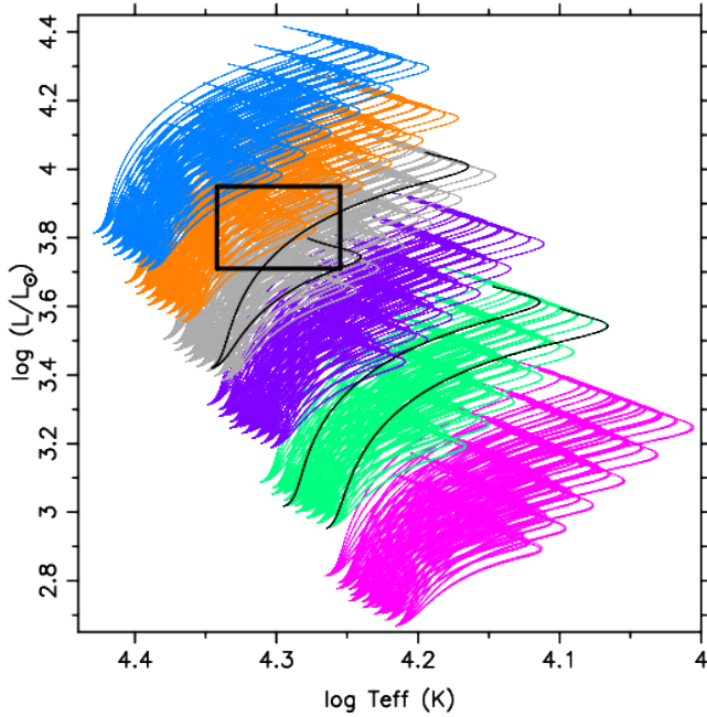
Fig. 4. Hertzsprung-Russell diagram with the 240 evolutionary tracks per mass in the SpaceInn grid for the masses 5 (pink), 6 (green), 7 (purple), 8 (grey), 9 (orange), and 10 (blue) M_{\odot} , along with the 2\sigma error box of HD 170580 based on Gaia DR2 data and spectroscopy. The pulsation modes of the four tracks in black are shown in Fig. 8.
