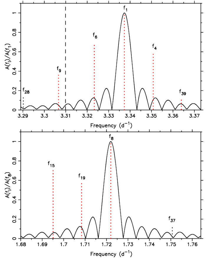
Fig. 3. Two zoomed parts of the amplitude spectrum, where the length of the x -axis equals ten times the Rayleigh limit. The spectral window (full line) is placed at the local dominant frequency (cf. Table 1). Dotted lines indicate the extracted frequencies whose amplitude was normalised to the dominant one in that frequency regime ( top panel: f_1 , bottom panel: f_8 ). Black dotted lines indicate combination frequencies. The dashed line in the upper panel is placed at the position where the fifth quintuplet component would occur in the case of equal splitting.
