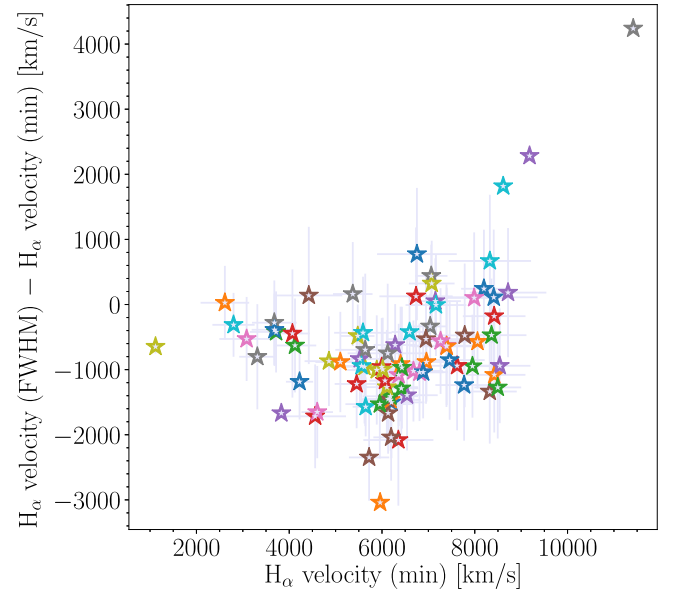
Figure 19. Shifts of the H_{\alpha} velocity obtained from the FWHM of the emission and from the minimum of the absorption at 50 days post-explosion.
