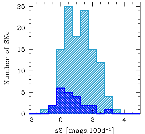
Figure 7. Distribution of the plateau decline s_2 in V band for 117 SNe of our sample. The blue histogram presents the distribution of “ s_2 ” in V band for 22 SNe II used as a new template in SNID.
