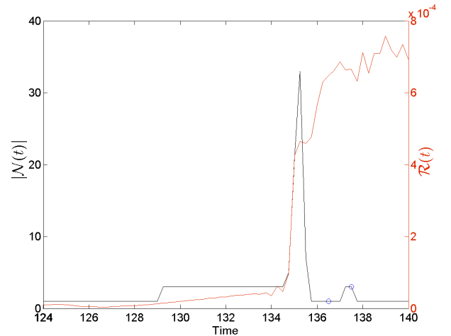
Fig. 9. Time series for |N(t)| (black) and \mathcal{R}(t) (red). Blue circles correspond to the connectivity maps (a) and (b) from Fig. 8. The y = 0 plane has been used as the initial location to trace field lines for the calculation of \mathcal{R}(t) .
