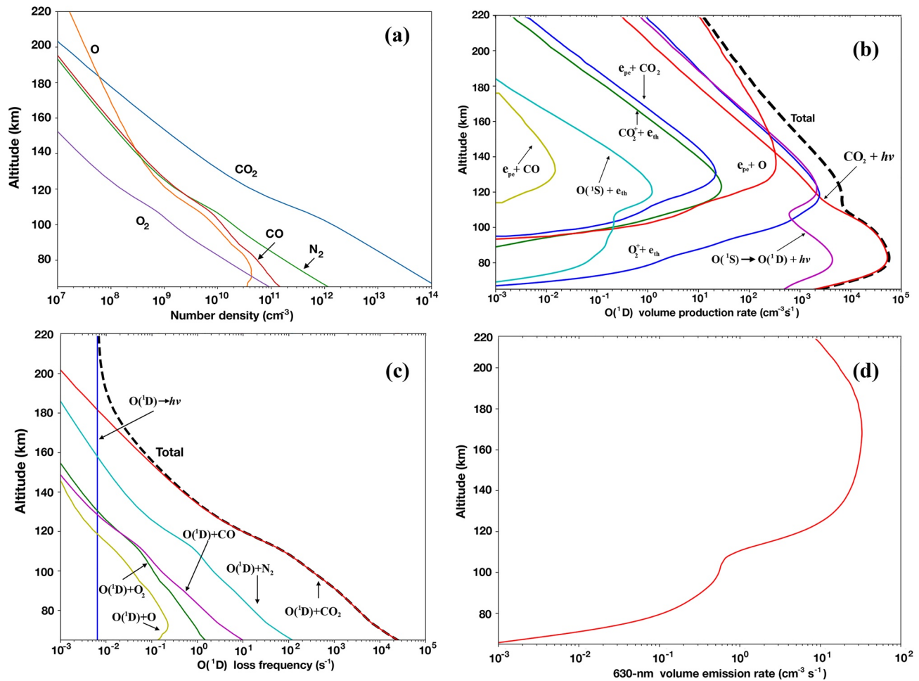
Figure 3. Altitude distribution of the number densities of neutral species (a), O(^1D) main sources (b), O(^1D) sinks (c), and 630 nm volume emission rate (d) in the Martian dayglow calculated for solar minimum conditions at aphelion, for a solar zenith angle of 30^\circ .
