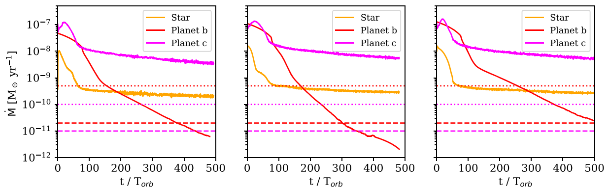
Figure 9. Accretion rates (in M_{\odot} \text{ yr}^{-1} ) on the sinks for all the simulations (left: Sim 1, middle: Sim 2, and right: Sim 3) as a function of the normalized time. Orange lines are the star accretion rate and red and pink lines are Planets b and c accretion rates, respectively. Horizontal red and pink dashed lines show the inferred values from Planets b and c respectively from Haffert et al. 2019, while the horizontal red and pink dotted lines show the inferred values from Planet b and c from Hashimoto et al. 2020.
