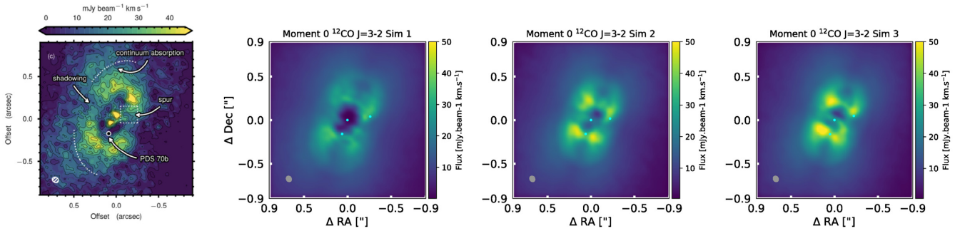
Figure 7. CO J = 3 - 2 integrated intensity (moment 0, continuum subtracted) for all the simulations for the t = 500 T_{\text{orb}} snapshot and, as a reference, the observed image of Kepler et al. (2019, left). The position of the star and the planets is shown as cyan dots. The image is convolved with a Gaussian 76 \times 61 mas beam with PA of 63^\circ as in Kepler et al. (2019) observations.
