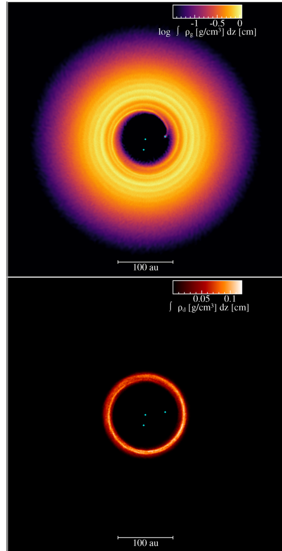
Figure 1. Top: logarithmic plot of the gas surface density map of the t = 500 T_{\text{orb}} ( \sim 0.18 \text{ Myr} ) snapshot for Sim 3. The blue dots are the positions of the star and the planets. Bottom: linear plot of the 1 mm dust surface density map of the t = 500 T_{\text{orb}} ( \sim 0.18 \text{ Myr} ) snapshot for Sim 3. The blue dots are the positions of the star and the planets.
