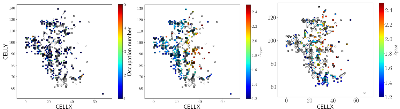
Fig. 6: Representation of SOM cells targeted by the KMOS programme. Left : coloured cells are filled with high-quality spectroscopic redshift measurements in the three fields targeted by our survey, whereas empty cells are occupied by observed and not spectroscopically confirmed targets. The high-quality spectroscopically assigned cells are colour-coded according to the occupation level, meaning the number of validated galaxies occupying the same colour cell. Middle : the SOM cells filled with high-quality spectroscopic redshift measurements are colour-coded according to the assigned z_{\text{spec}} . Right : the observed but still empty SOM cells are colour-coded according to the z_{\text{phot}} of the observed targets, whereas high-quality spectroscopic redshift measurements are coloured in white.
