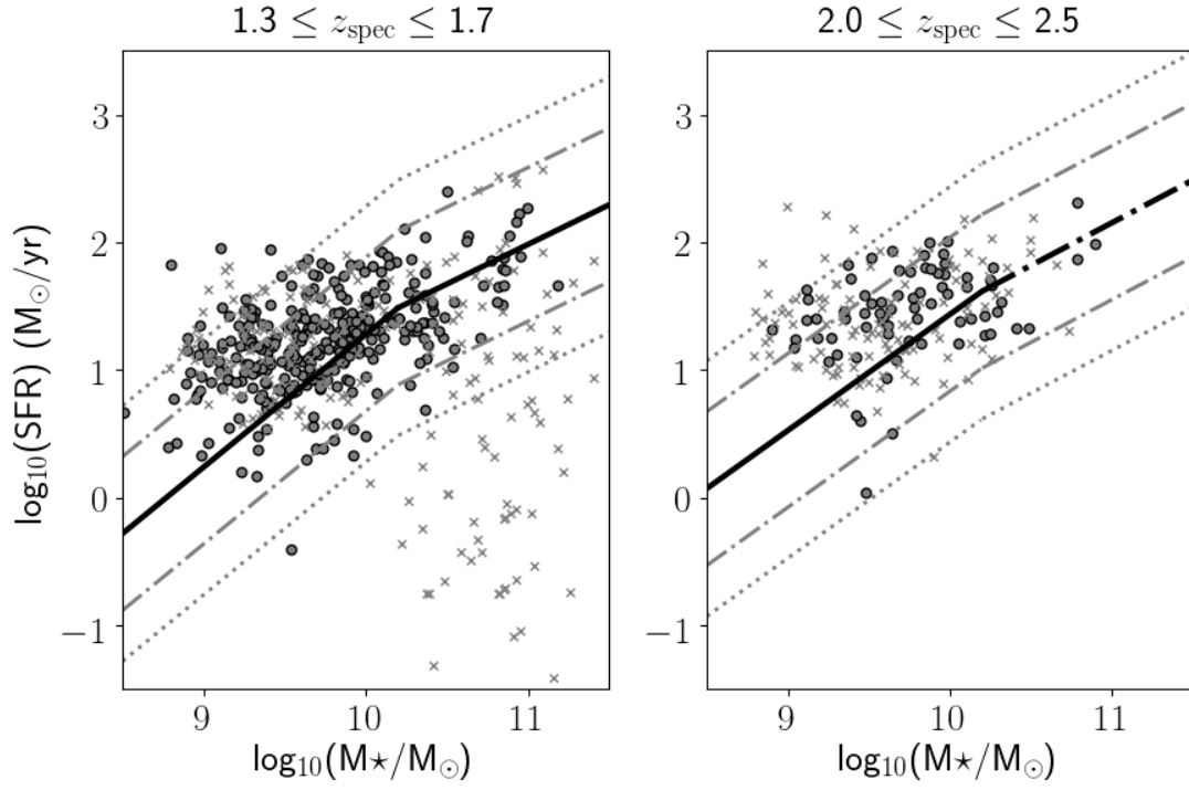
Fig. 12: ( H\alpha – based) SFR (grey circles) and (SED fitting based) SFR (grey crosses) vs stellar mass. The left panel shows the lower redshift targets observed in H -band in the three surveys considered in the scientific analysis presented here, and the right panel represents the same for higher redshift K -band targets. The black solid lines are the best fit to the star-forming main sequence (MS) in the same redshift range from Whitaker et al. (2014); the dashed and dotted lines show 4\times and 10\times above and below the MS and bracket the distribution of the data points of the 3D-HST galaxies (see Fig. 7 in Wisnioski et al. 2019).
