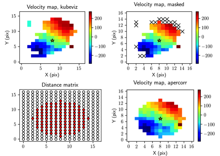
Fig. 9: Summary of procedure followed to estimate the H\alpha flux within the 1''.2 radius aperture, for a typical case of a galaxy with a rotation curve. The top-left panel shows the velocity map from KUBEVIZ. The star at the centre of the image represents the pixel position from which the aperture is estimated. The bottom-left panel shows the distance matrix that defines the six-pixel radius corresponding to the aperture. The top-right panel shows which spaxels from the original map are discarded because they fall outside the aperture. Finally, the bottom-right panel shows the corrected velocity field obtained following the procedure described in the main text for assigning a peculiar velocity to the spaxels flagged as bad in KUBEVIZ.
