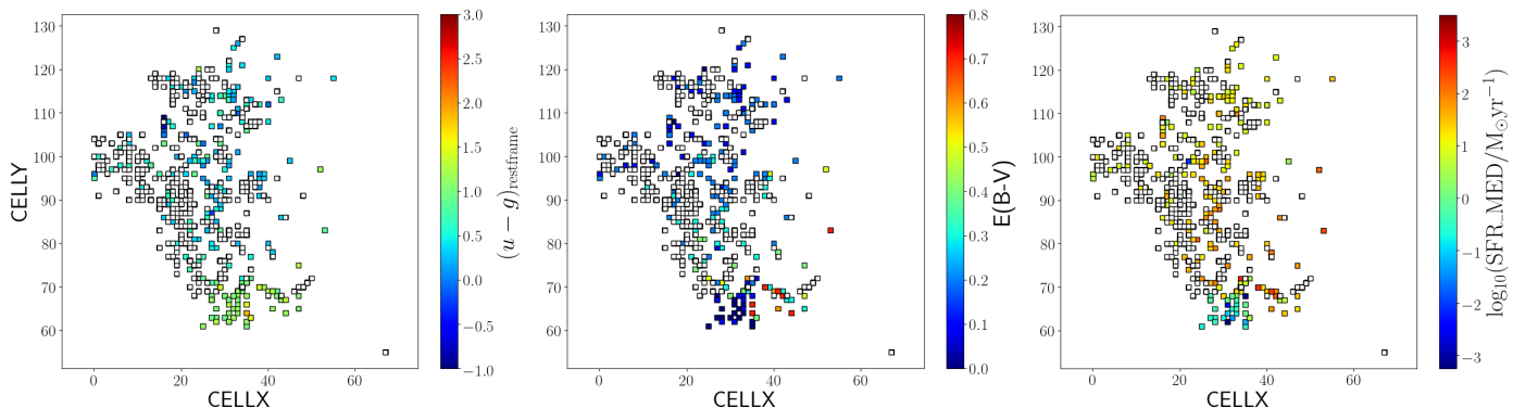
Fig. 7: Representation of SOM cells targeted by the KMOS programme. The cells filled with high-quality spectroscopic redshift measurements are coloured in white. Left : cells are colour-coded according to the restframe (u - g) colour. Middle : the cells are colour-coded according to the best fit E(B - V) resulting from SED fitting analysis on the photometric sample. Right : the cells are colour-coded according to the best fit SFR resulting from SED fitting analysis on the photometric sample.
