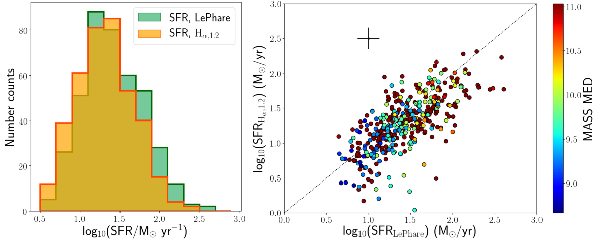
Fig. 11: Left : histogram of SFR derived from aperture H\alpha fluxes, and that estimated from LePhare SED fitting. Right : comparison between the H\alpha and SED-fitting SFRs, colour-coded by galaxy stellar mass. The black dashed line is the one-to-one correlation. The plot also shows the typical error on the SFR from LePhare (horizontal black error bar, calculated using the SFR_INF and SFR_SUP released in the catalogue) and on the H\alpha SFR (considering a typical uncertainty of 10% on the flux measurement, see Wisnioski et al. 2019).
