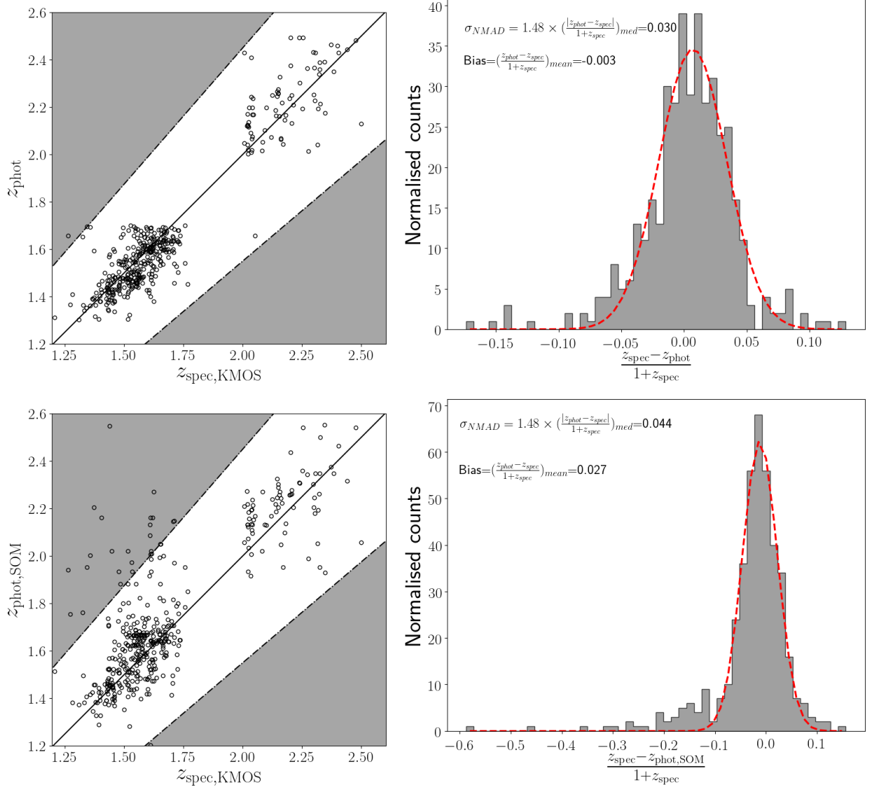
Fig. 2: Top left : comparison between z_{\text{phot}} and z_{\text{spec}} for high-quality ( Q \geq 3 ) redshift galaxies observed during the four periods of the KMOS Large Programme. Lower redshift targets are observed with the H -band grism, higher redshift ones with the K -band. The dashed lines define the region outside which the z_{\text{phot}} is considered a ‘catastrophic failure’ (grey area in the plot), defined by a redshift error |z_{\text{phot}} - z_{\text{spec}}|/(1 + z_{\text{spec}}) \geq 15\% . Top right : histogram of the (z_{\text{phot}} - z_{\text{spec}})/(1 + z_{\text{spec}}) of all high-quality redshift targets. A Gaussian with mean and sigma equal to the bias and \sigma_{\text{NMAD}} , respectively, is overplotted with a red dashed line. Bottom left : same as the top-left panel but comparing z_{\text{phot,SOM}} and z_{\text{spec}} . Bottom right : same as the top-right panel but with z_{\text{phot,SOM}} .
