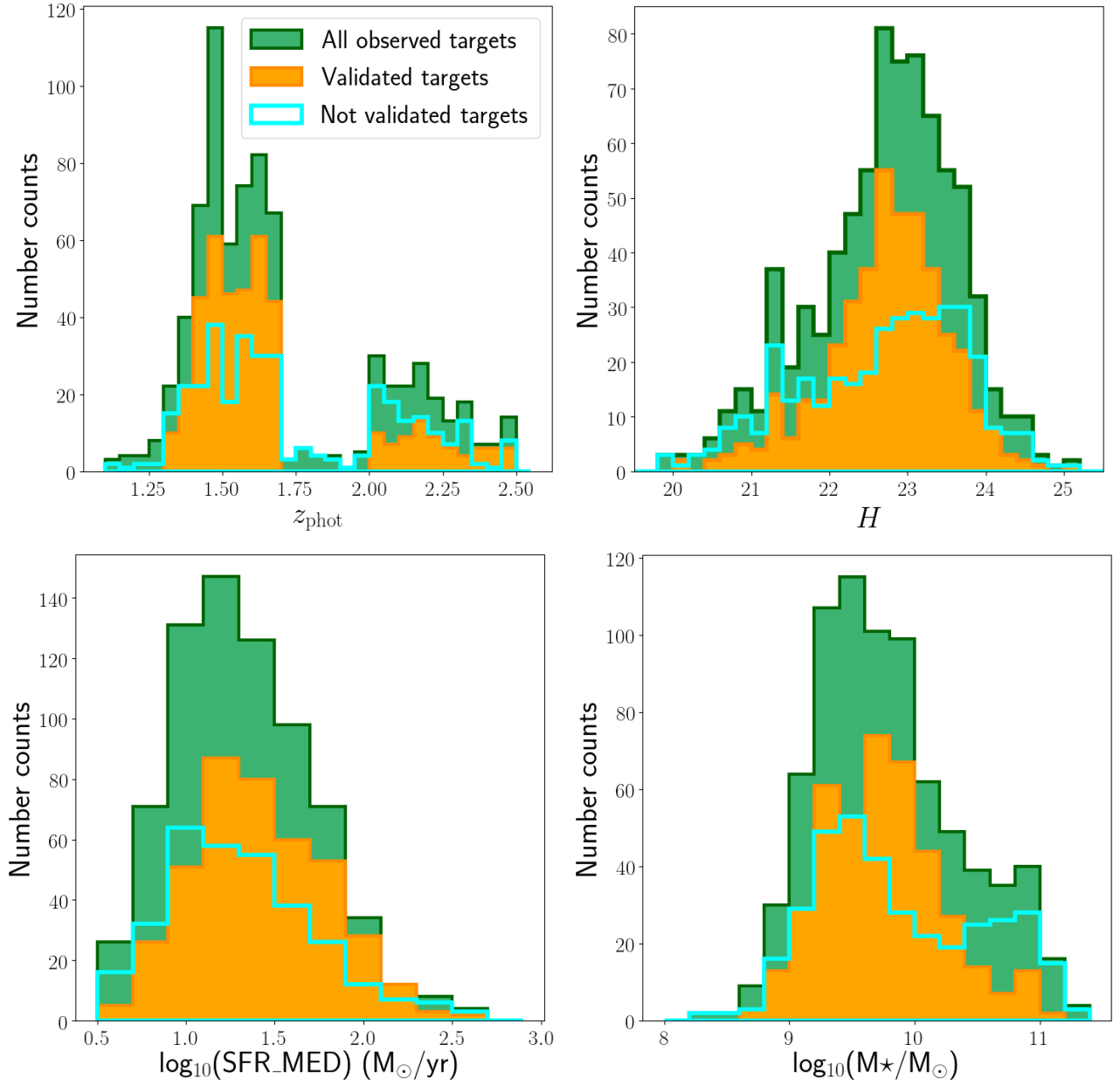
Fig. 5: Top Left : histogram of z_{\text{phot}} of individual galaxies from the literature. Top right : histogram of the observed H total magnitude for all observed targets (green filled), for those with high-quality spectroscopic redshifts (validated targets; orange filled) and for those that could not be assigned a spectroscopic redshift (not validated targets; open blue line). Bottom left : histogram of the SFR derived from SED fitting for the same samples. Bottom right : histogram of the stellar mass derived from SED fitting for the same samples.
