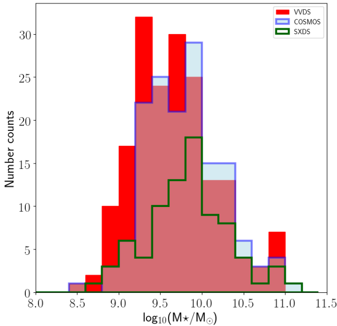
Fig. 8: Histogram of stellar masses computed by LePhare on the spectrophotometric catalogues ( z_{\text{spec}} sample) built in the three fields. The fields are shown with separate histograms as indicated by the legend.
