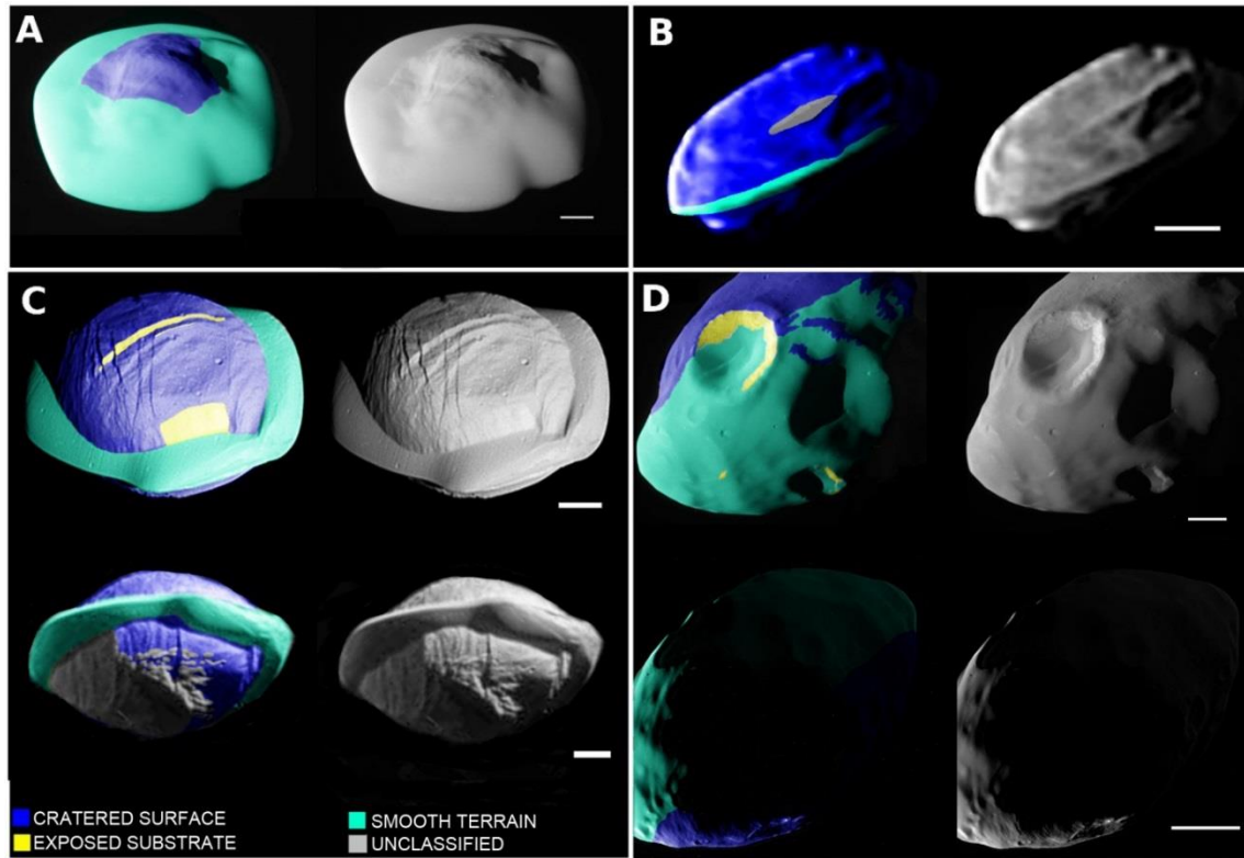
Fig. 3. Distribution of three primary units on ring moons (A) Atlas, scale bar 5 km. Obtained at 94m/pixel (m/p). (B) Daphnis, scale bar 2km; 167 m/p. (C) Pan scale bars 5 km; 144 m/p (top) and 279 m/p (bottom). (D) Pandora (top scalebar, 10km, bottom, 20 km); 137 m/p (top), 200 m/p (bottom). Cratered surface: heavy cratering, relatively crisp surface relief, and regolith typical of other small bodies in the Saturnian system. Smooth terrain: distinctly smooth compared to typical small body cratered surfaces; some is material collected in crater floors. Exposed substrate: relatively bright with lineations more typical of rigid materials than of loose regolith. Unclassified materials are those for which insufficient data are available to resolve ambiguities between terrain types.
