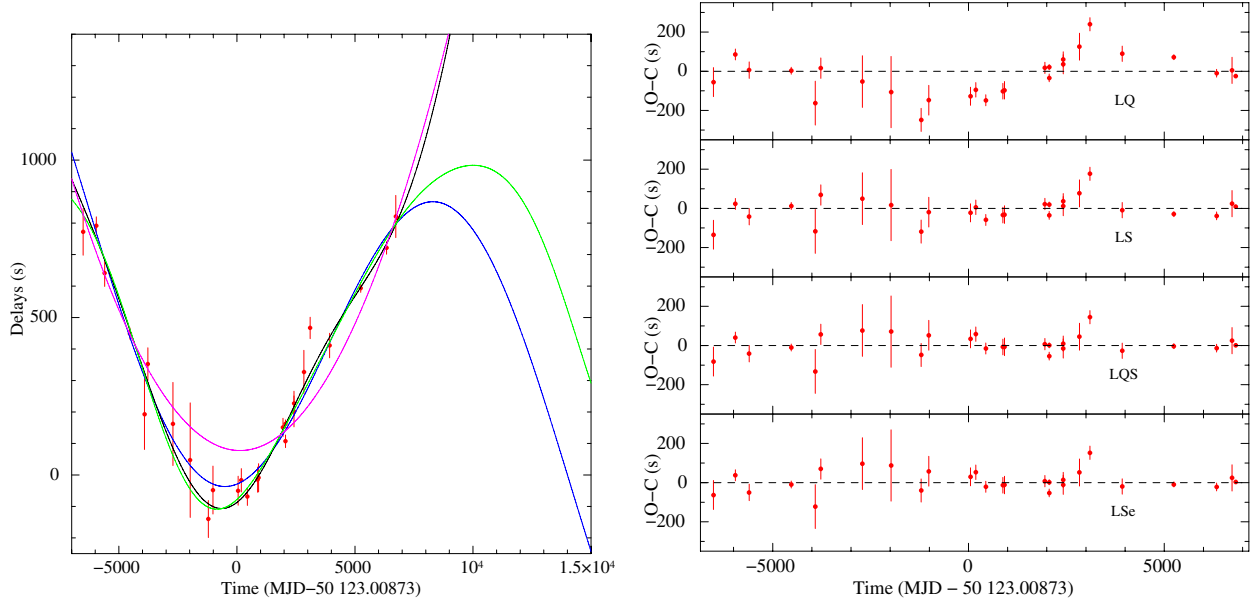
Fig. 3. Left panel: dips' arrival time delays versus time. The magenta, blue, black, and green curves are the best-fit curves obtained using the linear+quadratic (LQ), linear+sinusoidal (LS), linear+quadratic+sinusoidal (LQS), and linear+sinusoidal function taking into account a possible eccentricity (LSe), respectively. Right panel: observed minus calculated delays in units of seconds. The residuals, from the top to the bottom, correspond to the LQ, LS, LQS, and LSe function, respectively.
