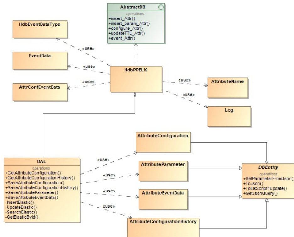
Figure 4. Class diagram.
