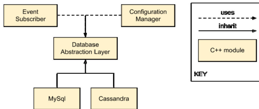
Figure 2. HDB++ Module View.
