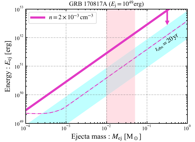
Figure 8. The same as Fig. 6 but for GRB 170817A. The pink and cyan shaded regions show the range of ejecta mass M_{\text{ej}} = 0.01-0.05 M_{\odot} and velocity \beta_{\text{in}} = 0.1-0.3 , respectively. The dash-dotted curve demonstrates how we can reduce the allowed region by late-time observations at 20 yr after the merger, assuming a tenfold improvement in sensitivity (e.g. Butler et al. 2018).
