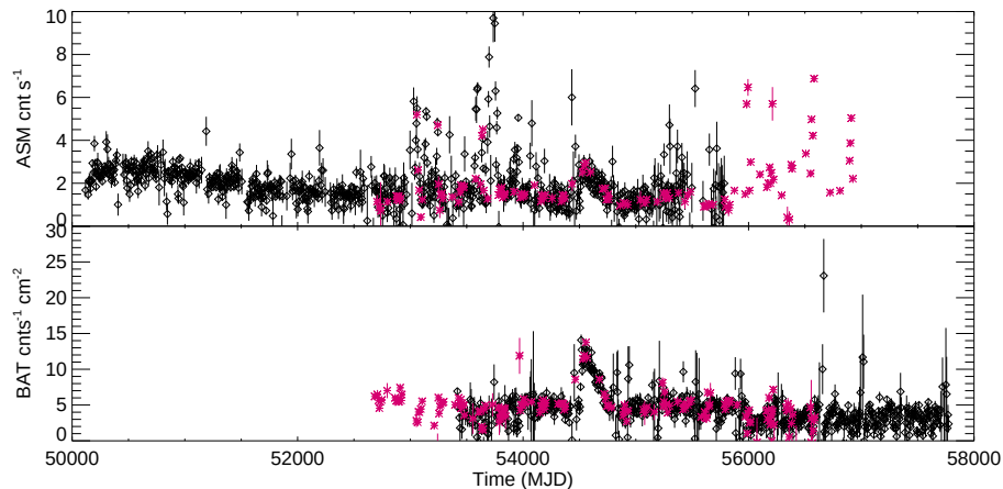
Figure 1. Top panel: ASM/RXTE 2–12 keV 10 days bin light curve of GRS 1724–308. The pink asterisks represent the INTEGRAL /JemX 2–12 keV 10 days bin light curve rescaled in arbitrary units. Bottom panel: Swift /BAT 15–50 keV 10 days bin light curve of GRS 1724–308. The pink asterisks represent the INTEGRAL /IBIS 20–100 keV 10 days bin light curve rescaled in arbitrary units.
