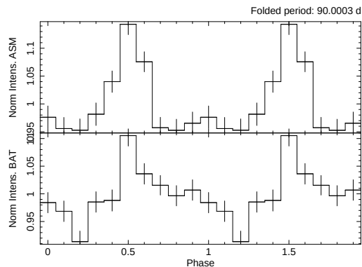
Figure 4. Top panel: ASM folded light curve of GRS 1724–308. The period corresponds to 90 days. Bottom panel: BAT folded light curve for the same period.
