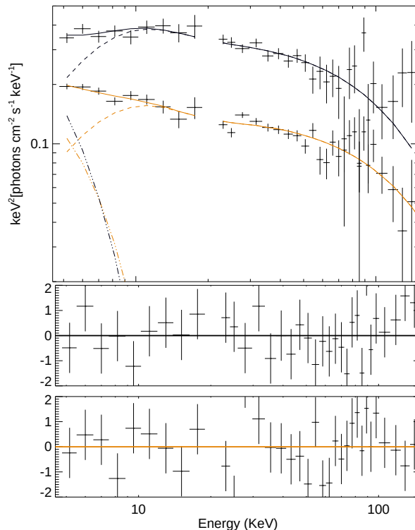
Figure 8. Top panel: GRS 1724–308 IBIS and JEM-X hard state unfolded spectra. The spectrum with orange lines corresponds to the orange points in Figure 6 (regular GRS 1724–308 hard state.) The spectrum with black lines corresponds to the black points in Figure 6 (2008 peculiar hard state) . Middle and bottom panel: respective fit residuals in terms of sigmas with error bars of size one.
