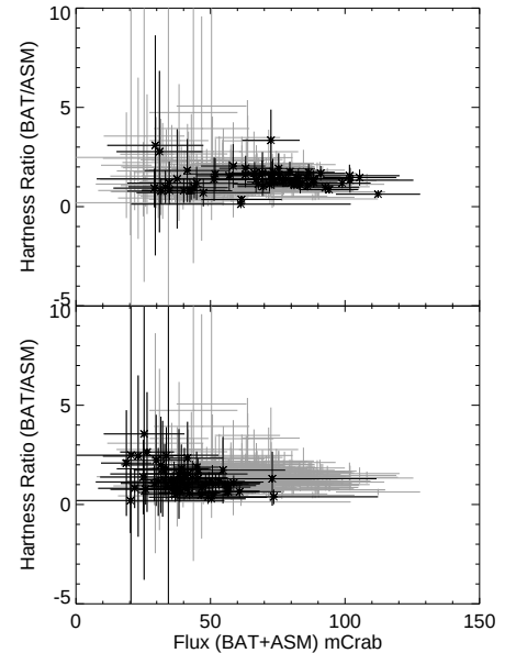
Figure 7. First panel: BAT/ASM HID of the entire 2008 peculiar flare (grey points). The black points represent the 1 st 60 days of the flare. As in the top panel, for the last 60 days of the flare (in black). Time range is (MJD)=54489–54781, bin time is 1 day (see also Fig 3 for light curve details)
