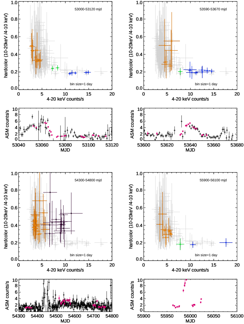
Figure 5. Jem-X color Intensity diagrams. The time bin of each point is equal to 1 day, the coloured points in each figure represent the evolution of the state transition of a single flare of the source. The points of the same colour represent the same spectral state (yellow for hard states, green for intermediate states and blue for soft and very soft states). Instead, the background grey data represent the whole dataset including the persistent emission. The black points represent the peculiar state observed only during the 2008 flare (for clarity these points were omitted in the background grey data, in order to highlight the ATOLL source HCI track of GRS 1724–308 ).
