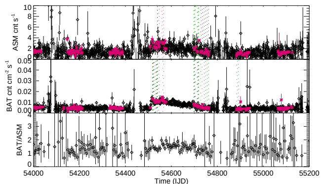
Figure 3. First two panels: ASM and BAT light curves as in Fig 1, but zoomed around the peculiar 2008 long flare (bin time 1 day). The green zones of the plots represent the INTEGRAL observing periods throughout the flare (during the periods represented with dashed zones the source has been observed only by IBIS, while during the dotted periods the source has been observed by both IBIS and JEMX). Bottom panel: ratio between BAT and ASM fluxes (bin time 5 day)
