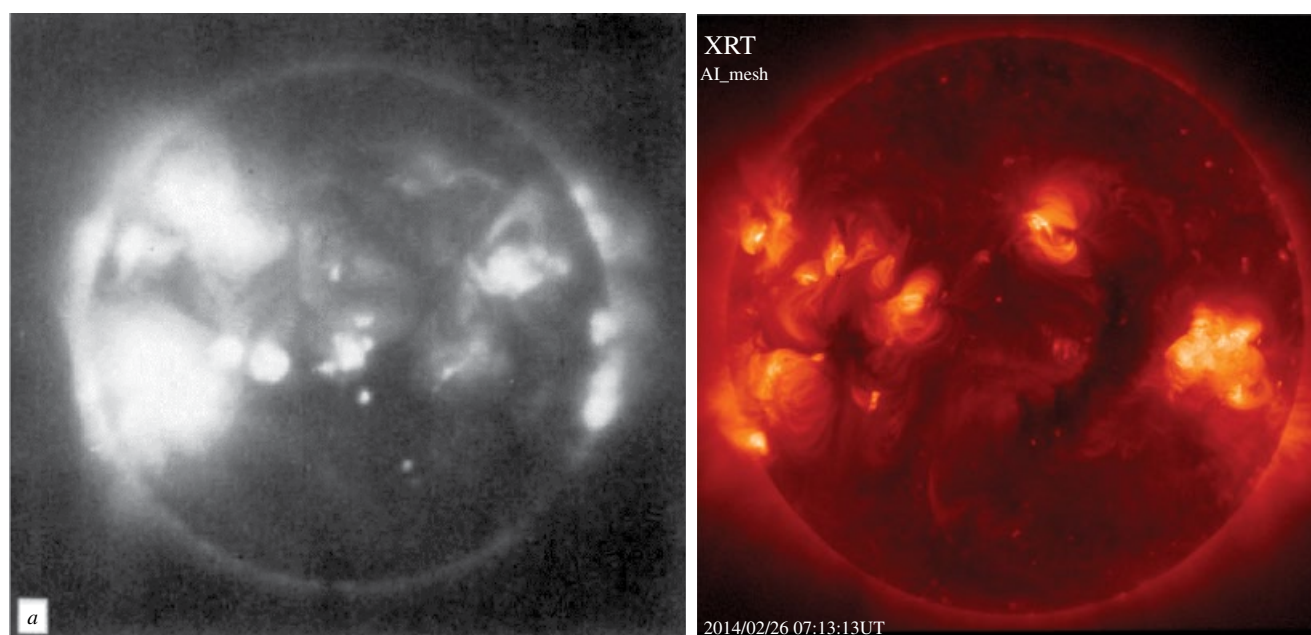
Figure 2.3 Left shows an X-ray image taken on 7 March 1970 from an Aerobee rocket; right shows an X-ray image taken on 26 February 2014, with Hinode XRT in the Al-mesh filter. (Source: (Left) Image from Van Speybroeck et al., 1970; (Right) Image courtesy of Smithsonian Center for Astrophysics, JAXA, and NASA.)
