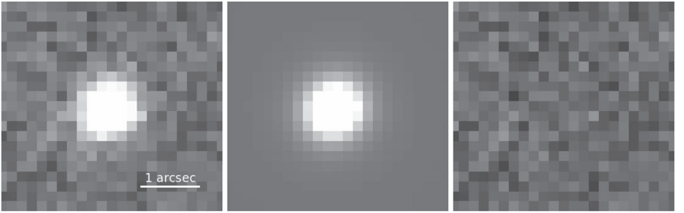
Figure 3. Panels show the i -band image from HSC, the best-fit galfit model, and residual, from left to right. The flux scales are the same in all the panels.
