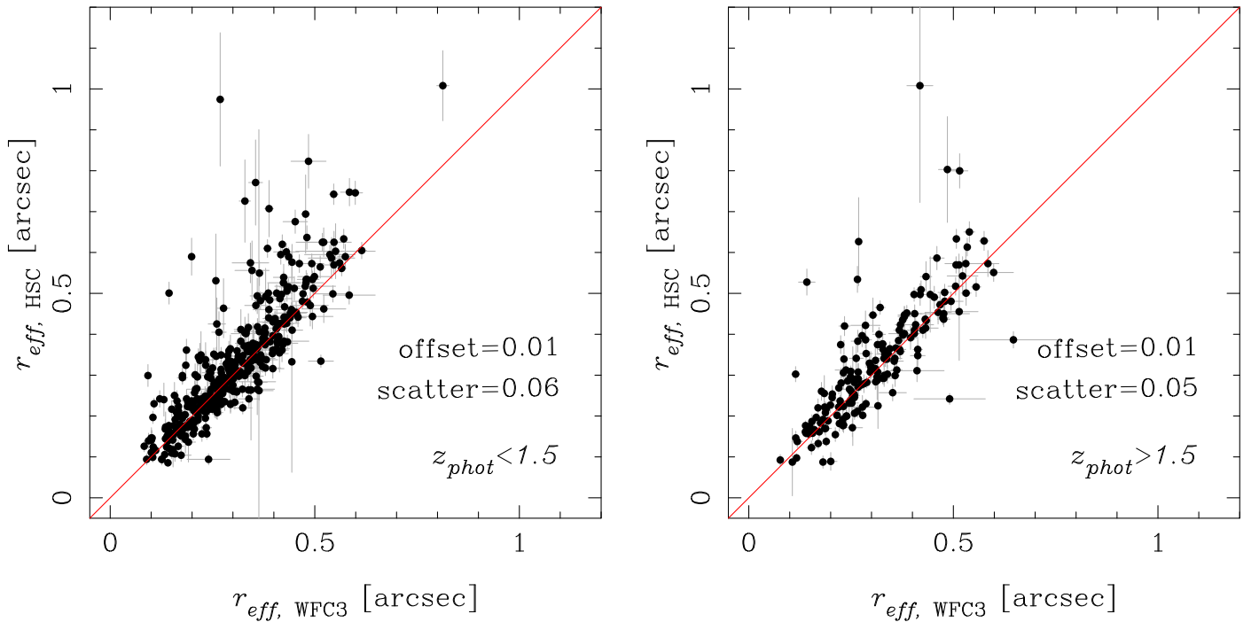
Figure 2. Size from HSC i -band plotted against size from HST F160W. The plotted objects have i -band magnitudes similar to that of the z = 4 object. The solid line shows r_{\text{eff, HSC}} = r_{\text{eff, HST}} . The left and right panels show objects at z < 1.5 and z > 1.5 , respectively. The systematic offset and scatter around it are shown in the figures.
