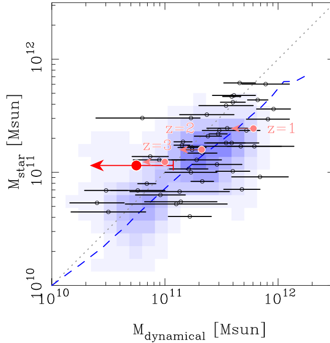
Figure 5. Left: stellar mass plotted against dynamical mass. The meaning of the symbols are the same as in the published article.
