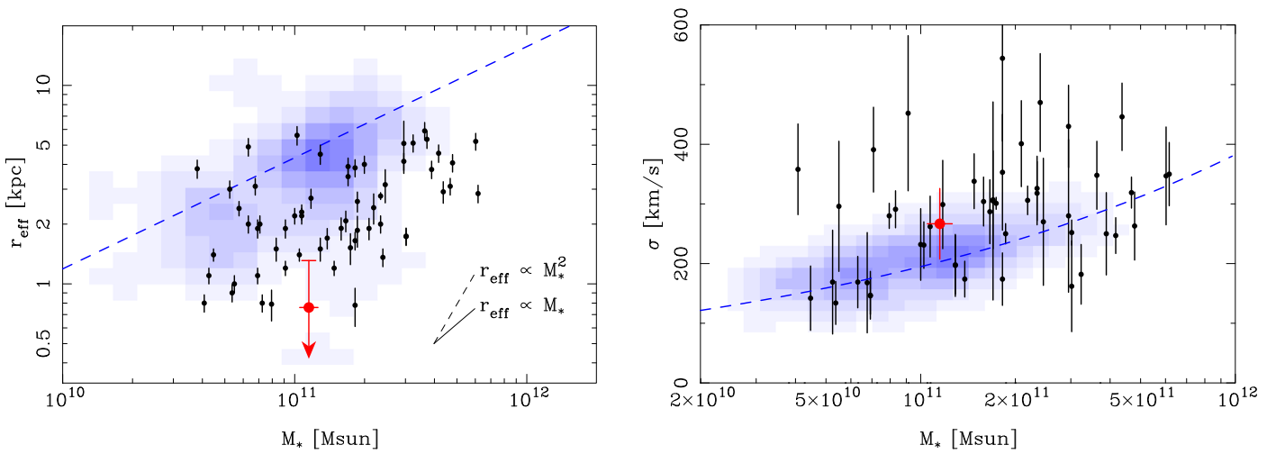
Figure 4. Left: size plotted against stellar mass. The z = 4 galaxy is shown in red. The black points are quiescent galaxies at z > 1.5 drawn from the literature; compilation by van de Sande et al. (2013), which includes van Dokkum et al. (2009), Onodera et al. (2012), Toft et al. (2012), Bezanson et al. (2013), and newer data from Belli et al. (2017) and Stockmann et al. (2019). Their mean redshift is around 2. The shades show data from the LEGA-C survey, which covers 0.6 \lesssim z \lesssim 1.0 . The dashed line shows the local relation from Shen et al. (2003) based on data from the Sloan Digital Sky Survey (SDSS; York et al. 2000; Strauss et al. 2002). The solid and dotted lines in the bottom right corner show evolutionary tracks with r_{\text{eff}} \propto M_* and r_{\text{eff}} \propto M_*^2 , respectively. They represent the major and minor merger tracks. Right: stellar velocity dispersion plotted against stellar mass. The meaning of the symbols are the same as in the left figure. The blue dashed curve is a fit to SDSS galaxies (Zahid et al. 2016).
