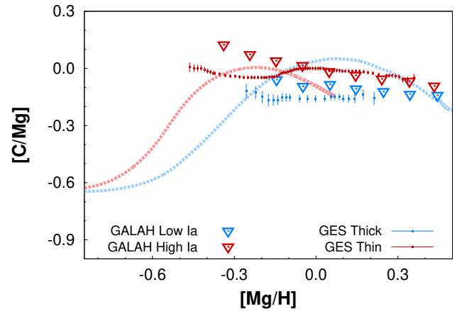
Fig. 6. [C/Mg] – [Mg/H] diagram. Data are from GES iDR5 and GALAH DR2 (dots and upside-down triangles, respectively) and include zero-point shifts (see text). Predicted trends for the thick (blue line) and thin (red line) discs are from the parallel model ( Grisoni et al. 2017 ) with the same nucleosynthesis prescriptions as model MWG-01 of Romano et al. (2019) .
