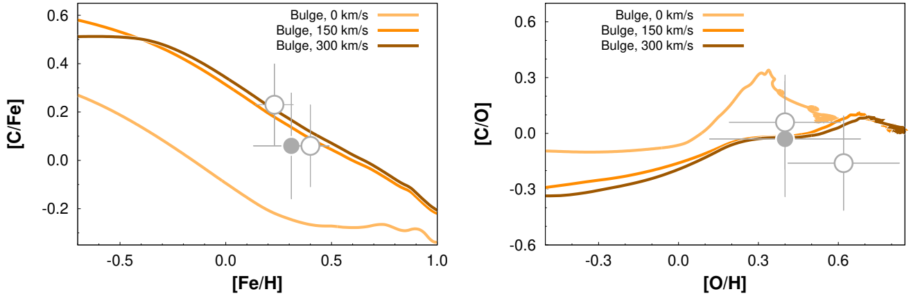
Fig. 7. Carbon-to-iron ( left panel ) and carbon-to-oxygen ( right panel ) abundance ratios as functions of [\text{Fe}/\text{H}] and [\text{O}/\text{H}] , respectively, in the Galactic bulge. The solid lines show the predictions of the chemical evolution model for the bulge by Matteucci et al. (2019) , including the same nucleosynthesis prescriptions as models MWG-05 (brown), MWG-06 (orange), and MWG-07 (yellow) of Romano et al. (2019) . Data for microlensed bulge dwarfs from Johnson et al. (2008) , filled circles) and Cohen et al. (2009) , empty circles) are also shown. All abundance ratios were normalised to the solar photospheric abundances by Asplund et al. (2009) .
