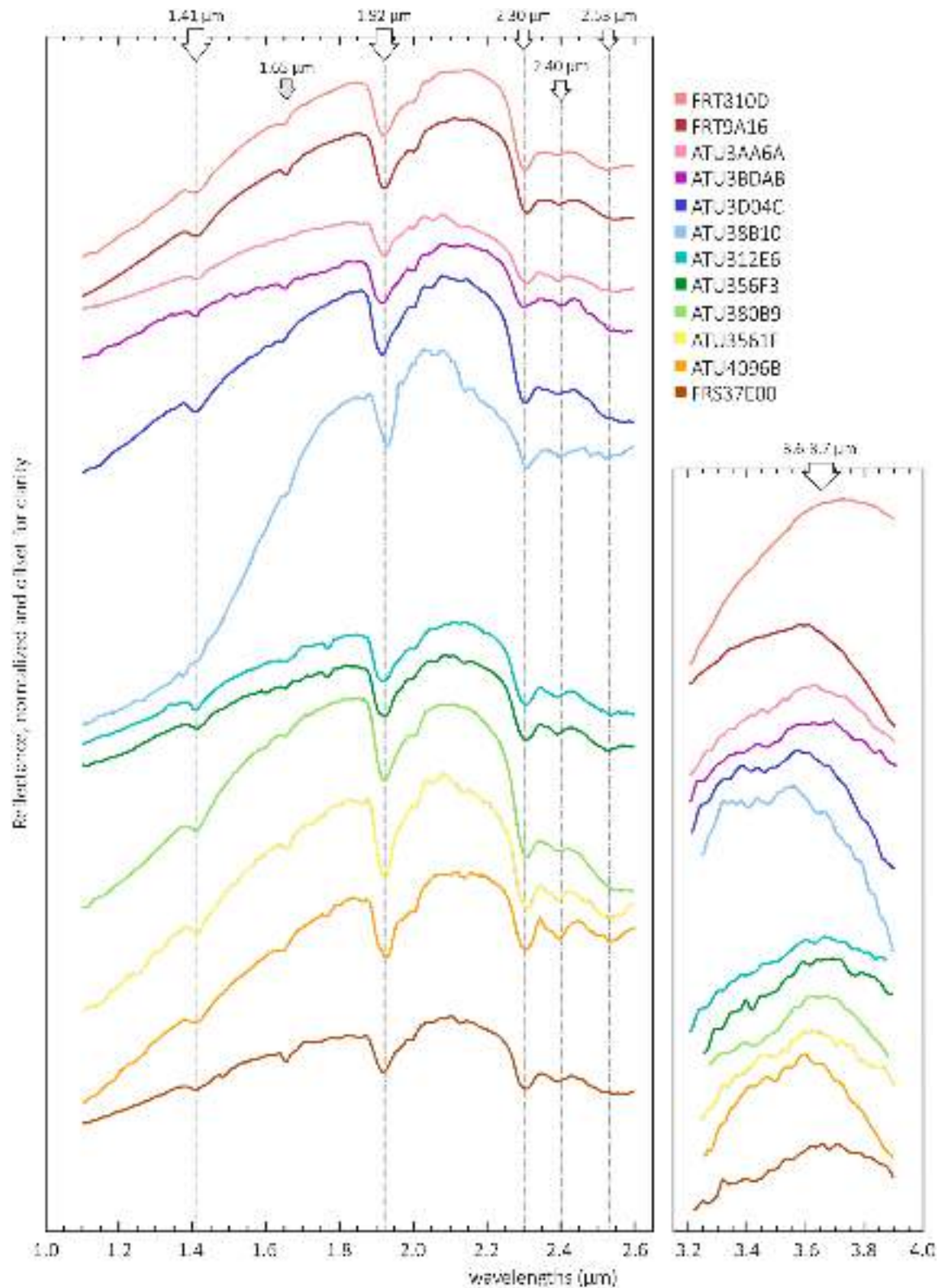
Fig. 8. Spectra of the CRISM denoised reflectance, normalized and offset for clarity. Unusable data at (1) 1.65 \mu\text{m} is associated with intermittent spikes from a detector filter boundary, (2) 2.60–2.80 \mu\text{m} is due to a saturated atmospheric \text{CO}_2 absorption there, and (3) 3.18 \mu\text{m} is an instrumental artifact (Murchie et al., 2007, 2009). Spectra are smoothed by averaging hundreds to thousands of pixels (Table 2). All spectra (notably ATU38B10) have a positive slope in the 1–2 \mu\text{m} range, likely due to the broad 1.2 \mu\text{m} absorption of a ferrous component (e.g., Bishop et al., 2008; McKeown et al., 2009). They all exhibit a broad “bulge-like” feature near 3.6–3.7 \mu\text{m} , typical of Martian carbonates (e.g., Bultel et al., 2019).
