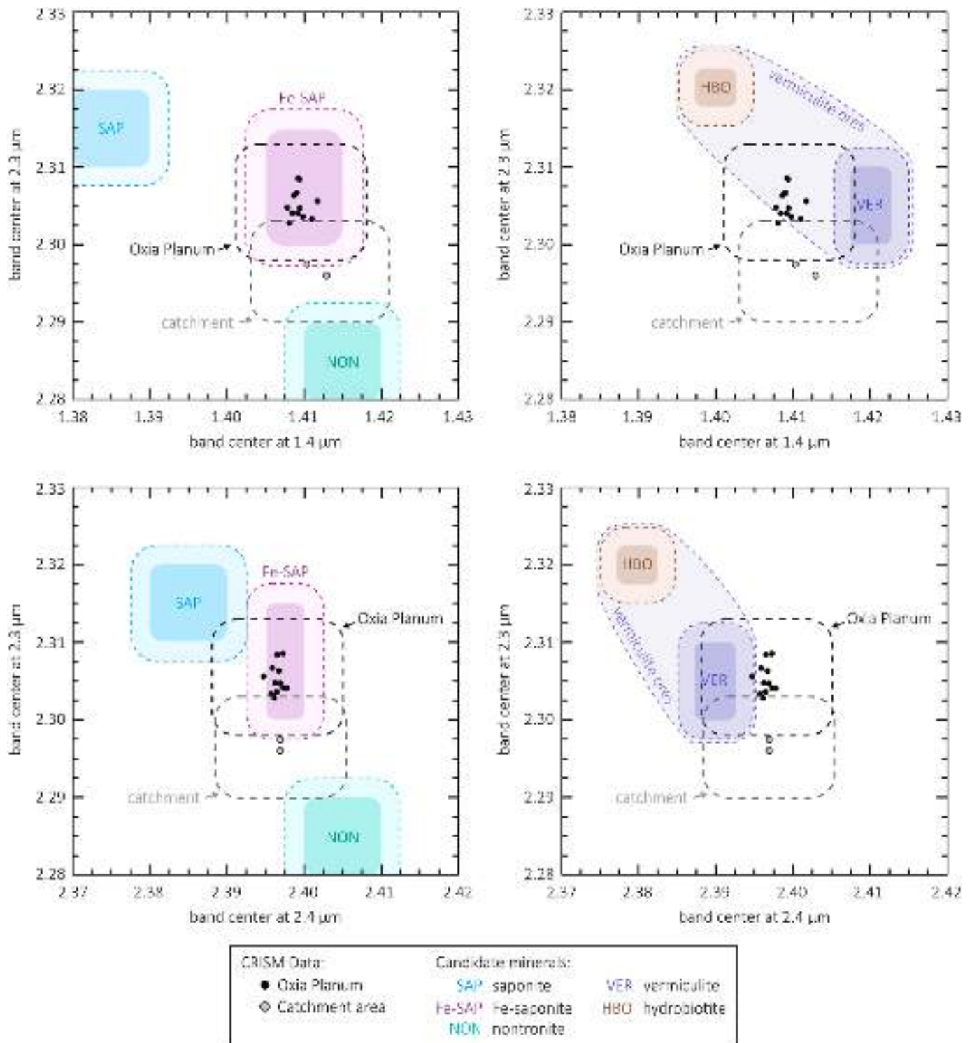
Fig. 9. (top) Scatterplots of 2.3 \mu\text{m} vs 1.4 \mu\text{m} band centers for the studied clay-bearing outcrops and candidate clays: nontronite and saponite (Clark et al., 1990; Bishop et al., 2013a), Fe-rich saponite (Treiman et al., 2014), and vermiculite ores (including pure vermiculite and hydrobiotite components separately) (Swayze et al., 2018a). (bottom) Scatterplots of 2.3 \mu\text{m} vs 2.4 \mu\text{m} band centers. Clay-bearing outcrops in Oxis display strong correlation with Fe-rich saponite (left panels) and also vermiculite ores (right panels), while outcrops identified in the catchment area are rather consistent with nontronites. Dashed outlines indicate the error areas: 2.5 nm for the candidate minerals (sampling) and standard deviations for the CRISM data analyzed here (Table 2).
