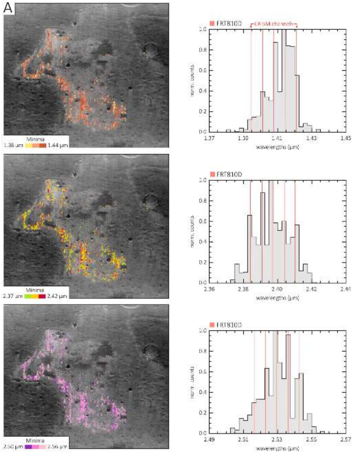
Fig. 4. (A) FRT810D cube near the landing ellipse center (335.5°E, 18.2°N): (left) Maps displaying the distribution of the diverse centers around 1.4 \mu\text{m} (1.37–1.45 \mu\text{m} ), 2.4 \mu\text{m} (2.36–2.44 \mu\text{m} ) and 2.5 \mu\text{m} (2.49–2.57 \mu\text{m} ), which are subdivided into 3 classes. At 1.4 \mu\text{m} : (1) below 1.40 \mu\text{m} , (2) between 1.40 and 1.41 \mu\text{m} , and (3) above 1.41 \mu\text{m} . At 2.4 \mu\text{m} : (1) below 2.39 \mu\text{m} , (2) between 2.39 and 2.40 \mu\text{m} , and (3) above 2.40 \mu\text{m} . At 2.5 \mu\text{m} : (1) below 2.52 \mu\text{m} , (2) between 2.52 and 2.54 \mu\text{m} , and (3) above 2.54 \mu\text{m} .
