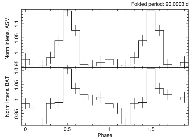
Figure 4. Top panel: ASM folded light curve of GRS 1724–308. The period corresponds to 90 d. Bottom panel: BAT folded light curve for the same period.
