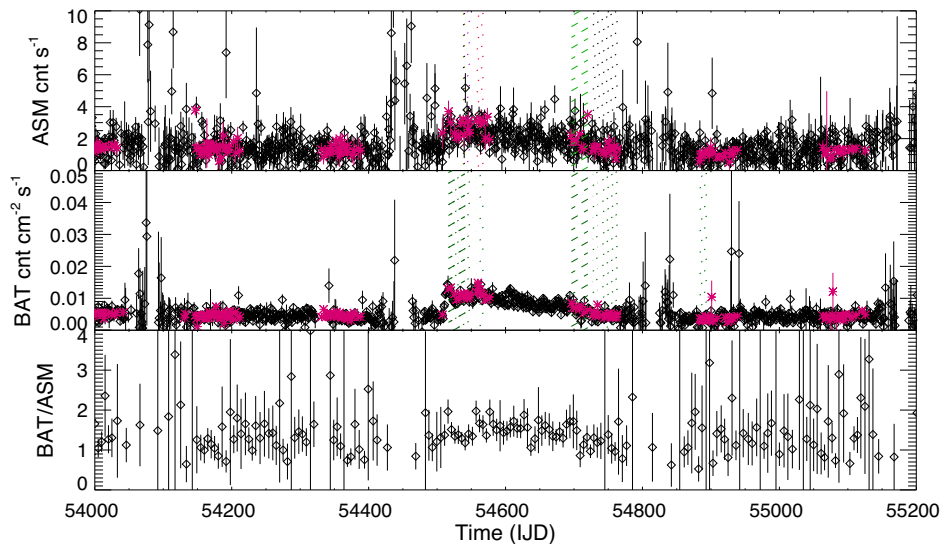
Figure 3. First two panels: ASM and BAT light curves as in Fig. 1, but zoomed around the peculiar 2008 long flare (bin time 1 d). The green zones of the plots represent the INTEGRAL observing periods throughout the flare (during the periods represented with dashed zones the source has been observed only by IBIS, while during the dotted periods the source has been observed by both IBIS and JEMX). Bottom panel: ratio between BAT and ASM fluxes (bin time 5 d)
