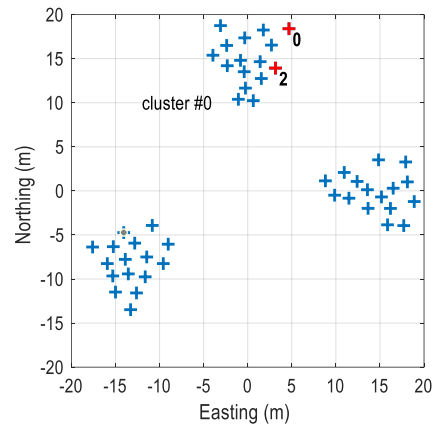
Figure 3. Layout of AAVS1.5. Antennas #0 and #2 of cluster #0 highlighted.
