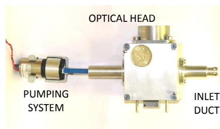
Fig. 2. MicroMED breadboard.
