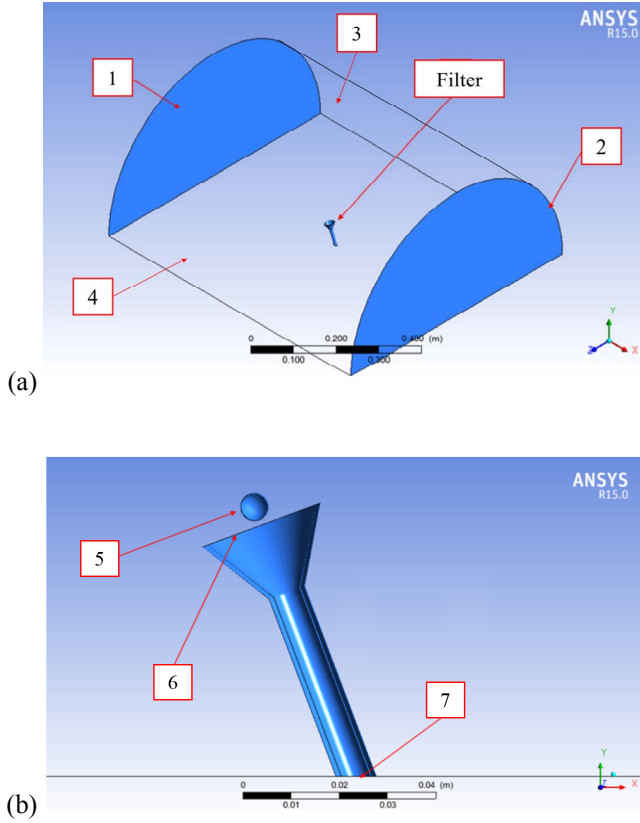
Fig. 4. Sketch of the computational domain: (a) overall view (b) detailed view of the filter
