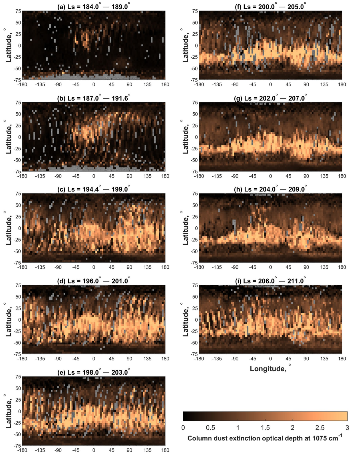
Figure 4. The evolution of the global dust storm of Martian Year 34. The diurnally averaged spatial maps of column dust extinction optical depth at 1,075\text{ cm}^{-1} in the periods: (a) from L_s = 184.0^\circ to L_s = 189.0^\circ , (b) from L_s = 187.0^\circ to L_s = 191.6^\circ , (c) from L_s = 194.4^\circ to L_s = 199.0^\circ , (d) from L_s = 196.0^\circ to L_s = 201.0^\circ , (e) from L_s = 198.0^\circ to L_s = 203.0^\circ , (f) from L_s = 200.0^\circ to L_s = 205.0^\circ , (g) from L_s = 202.0^\circ to L_s = 207.0^\circ , (h) from L_s = 204.0^\circ to L_s = 209.0^\circ , (i) from L_s = 206.0^\circ to L_s = 211.0^\circ .
