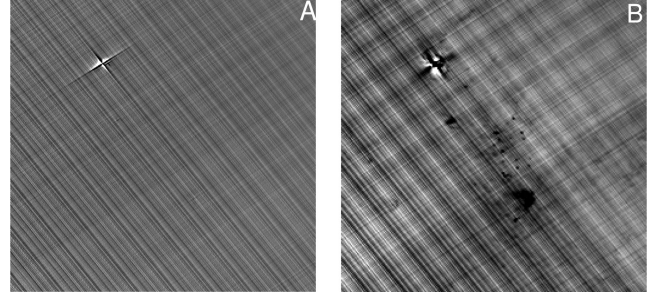
Figure 12. Difference of GLS and naive maps, \mathbf{e}_g , for the Rosette patch in the blue band (plot A) and red band (plot B). The 1/f noise is seen as the stripes following the scan lines. Comparing with Fig. 11 we see that the cross-like artefact present in the GLS map is clearly visible. Signal dependent distortion is also there in the red band but it is diffuse and not cross-like.
