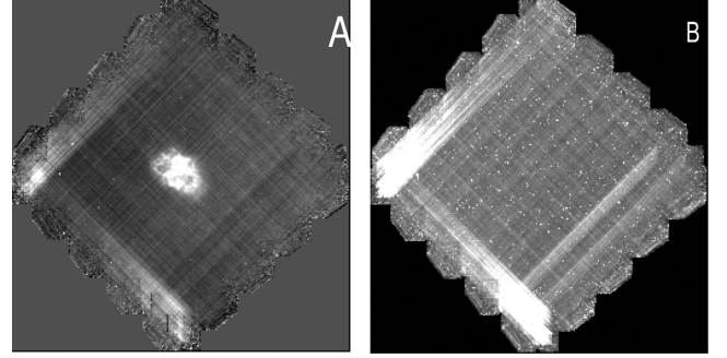
Figure 2. Images of the Crab nebula in the red band. The image is obtained by two, orthogonal scans. Plot (A) shows the N0 map and plot (B) shows the corresponding noise map. Several disturbances are clearly seen. The onset at the beginning of each scan is visible in the left-hand and lower corners. A jump involving an entire array row, starting near the right-hand corner, is seen in the noise map and, to a lesser extent, also in the naive map. Several glitches can be seen in the naive map as bright, isolated pixels and even more can be seen in the noise map. The stripes following the scan lines are due to the 1/f noise. The drift is almost absent.
