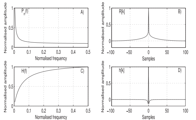
Figure 7. Plot (A) reports an example of noise spectrum P_n(f) following the model of equation (8). Plot (B) the corresponding autocorrelation sequence R[k] . Plot (C) is the reciprocal of the spectrum H(f) and plot (D) reports the noise filter response h[k] . Since P_n(0) = \infty , reflecting the fact that the timeline is affected by an unknown offset, we set H(0) = 0 and the correlation base to zero.
