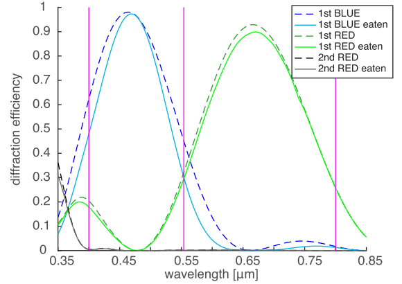
Figure 6. Diffraction efficiencies of the gratings composing the multiplexed element. The dotted lines refer to the single-layer efficiencies (first and second diffraction orders), while the solid lines refer to the corrected efficiencies (labelled ‘eaten’) at the exit of the multiplexed element, due to the reciprocal interference of the dispersive layers. Vertical lines identify the wavelength boundaries of the spectra in the CCD for each VPHG. ‘Blue 2’ is a VPHG with \Delta n = 0.038 and d = 6 \mu\text{m} , while ‘Red 2’ with \Delta n = 0.024 , d = 12 \mu\text{m} and \phi = 0^\circ 5 .
