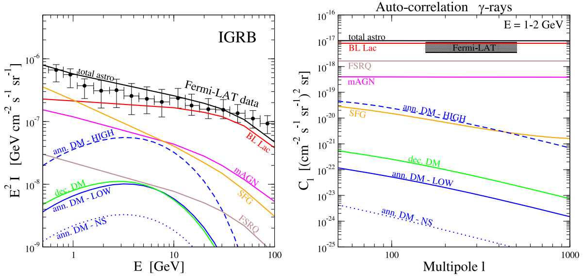
Figure 1. Average gamma-ray intensity I_\gamma as a function of photon energy (left) and auto-correlation APS C_l^{(\gamma)} in the (1–2) GeV energy band (right) for the benchmark \gamma -ray models considered in this work. The black lines denote the total contribution arising from astrophysical sources (i.e., the sum of BL Lac, mAGN, FSRQ, and SFG emission). Fermi -LAT data are shown as black points (left, from Ackermann et al. 2015a, adding in quadrature systematic and statistical uncertainties) and a shaded region (right, from Ackermann et al. 2012a, including the measurements with and without foreground cleaning).
