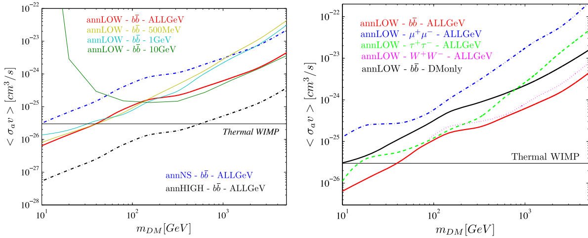
Figure 10. Left: 95% upper bounds on the DM annihilation rate \langle \sigma_a v \rangle as a function of the DM mass, for the LOW substructures model and the reference NVSS-10 A_{\text{th}}^k \neq 0 fit. Solid lines refer to the b\bar{b} annihilation channel: the red line refers to the analysis that combines information from all the three energy bins under consideration ( E > 0.5, 1, 10 GeV), while the other three lines refer to the analysis performed on a single energy bin (as stated in the figure label). The upper dotted-dashed blue line refers to the NS substructure model, while the lower dotted-dashed black line to the HIGH substructure model. Right: in addition to the b\bar{b} case (red line) reported in the left panel, the different lines show the upper bounds for the \mu^+\mu^- (blue), \tau^+\tau^- (green), and W^+W^- (magenta) annihilation channels, for the LOW substructures model. The black line instead shows the upper bound for the b\bar{b} case and LOW substructure scheme, obtained under the assumption that the DM contribution to the 2MASS cross-correlation is the dominant one (taken from Regis et al. 2015).
