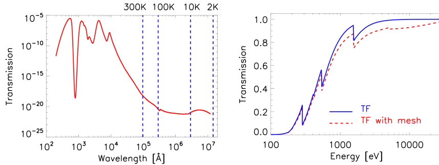
Fig. 1 UV/VIS/IR transmission ( left ) for a set of five TF with a total of 225 nm polyimide and 150 nm Al. X-ray transmission ( right ) for the same set of TF without meshes ( solid line ) and with a 96% open area Ti mesh on two filters ( dashed line ). Color figure online
