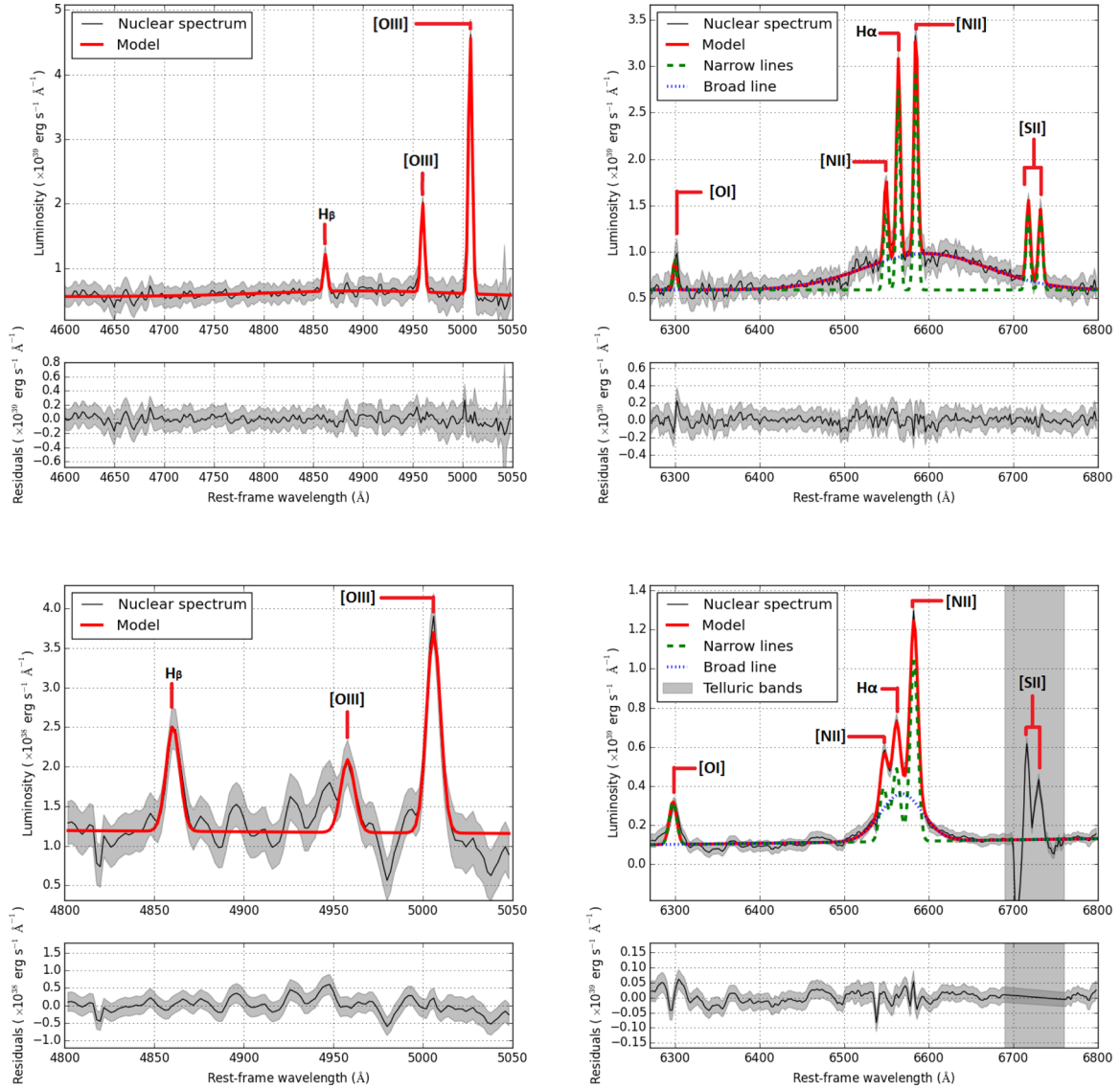
Figure 4. Top: decomposition of the AGN emission into continuum plus narrow and broad emission lines for J00 (top) and J02 (bottom). Left-hand panels: H\beta + [O III] region. Right-hand panels: H\alpha region. In grey, we plot the error of each spectrum. We also indicate the observed narrow emission lines.
