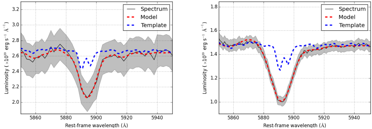
Figure 5. Spectrum (in black) of the Na I Doublet of J00 (left) and J02 (right) and its fit (in red). In grey we show the error of each spectrum. In blue we plot the template used to measure \sigma_e in the region of Na I D. The template has a spectral resolution of 1.28 \text{ \AA} .
