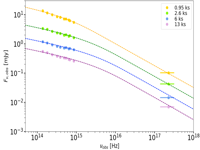
Fig. 3. The four spectral energy distributions estimated at T_{\text{mid}} . De-reddened optical data and un-absorbed X-ray flux are shown. Dashed lines represent our fitting model.
