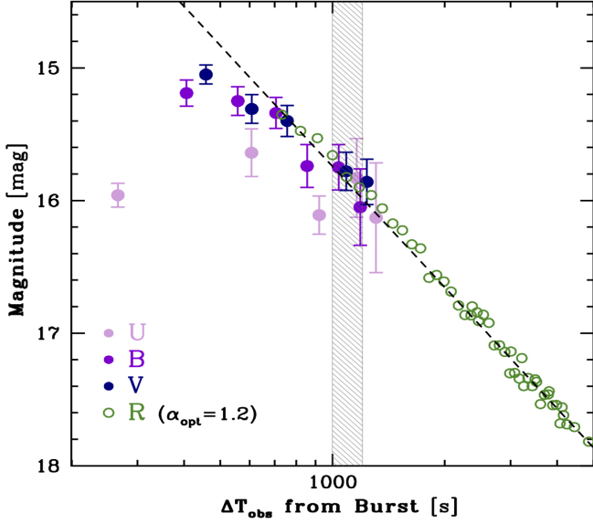
Fig. 2. Early time UVB magnitudes normalised to the R -band light curve at t \sim 10^3 s (shaded region). The dashed line is the power-law decay index of the late time optical afterglow.
