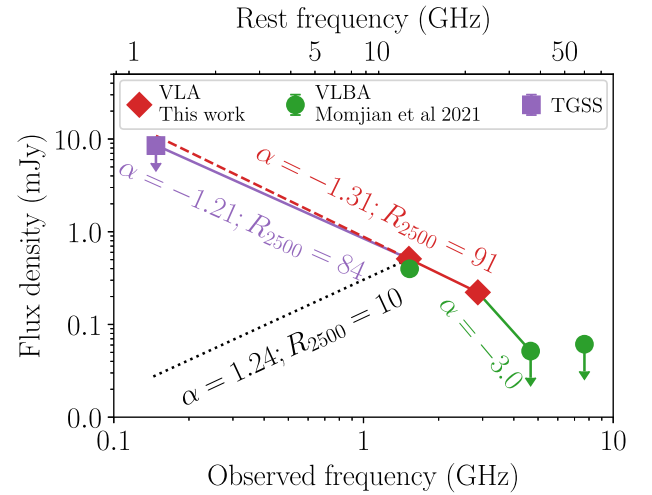
Figure 6. Radio spectral energy distribution of P172+18, including data from our VLA follow-up observations (red diamond), the VLBI measurements (green circles) from Momjian et al. (2021), and a 3\sigma upper limit from the TGSS (purple square). The power-law index, \alpha , is shown between the measurements as well as the radio-loudness by extrapolating the radio emission to rest-frame 5 GHz. The dotted line with \alpha = 1.24 represents the turnover required for P172+18 to be classified as radio-quiet (i.e., R_{2500} < 10 ).
