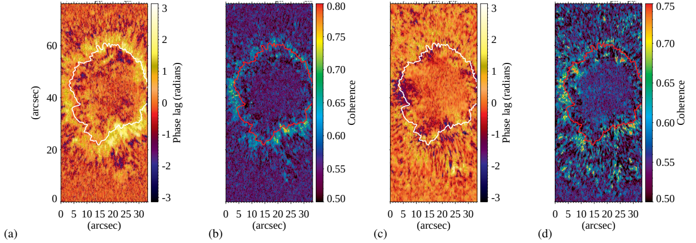
Figure 2. (a) Phase lag map of CP fluctuations at 3 mHz (with a bandwidth of 0.7 mHz) between the photosphere and chromosphere. (b) Coherence map at 3 mHz (with a bandwidth of 0.7 mHz) for the same CP disturbances. (c) Phase lag map at the same frequency band computed between CP fluctuations and core intensity fluctuations in the photosphere. (d) Coherence map corresponding to the phase map of panel (c). The continuous contours indicate the approximate position of the umbra-penumbra boundary as seen in the continuum intensity. The dashed lines highlight the region where the analysis was performed (see text for more details). Please note that the maps are obtained by averaging four spectral bins in Fourier space or, equivalently, 3.0 \pm 0.7 mHz. For this reason, the average phase and coherence values might appear lower than they are at each frequency bin.
