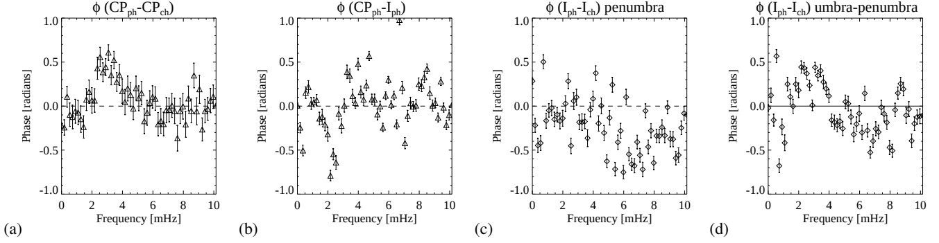
Figure 3. (a) Phase lag diagram between the CP signals in the photosphere and chromosphere computed in the annular region highlighted by the dashed lines in panel (b) of Fig. 2. (b) CP -Intensity phase diagram in the annular region of Fig. 2 panel (b) estimated in the photosphere. All plots are obtained by considering only those phase values for which the coherence is larger than 95% in each frequency bin. (c) Phase lag diagram of intensity perturbations in the core of the Fe I 617.3 nm and Ca II 854.2 nm spectral lines in the penumbra outside the annular region of panel (b) Fig. 2. (d) Phase lag diagram between intensity perturbations in the core of the Fe I 617.3 nm and Ca II 854.2 nm spectral lines. The diagram is obtained in the annular region highlighted by the dashed lines in panel (b) of Fig. 2.
