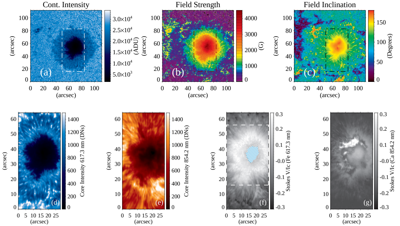
Figure 1. SOT/SP continuum intensity (panel a), magnetic field strength (panel b) and inclination (panel c) from HINODE level 2 data products. The dot-dashed rectangular box represents the IBIS FoV. (Panels d and e): IBIS intensity images in the core of the Fe I 617.3 nm line and of the Ca II 854.2 nm line, respectively. (Panel f): CP map obtained from the IBIS Fe I 617.3 nm line measurements. The central region of the umbra that is affected by possible saturation effects and low photon flux is indicated as a hatched area. (Panel g): CP map derived from the IBIS Ca II 854.2 nm line data.
