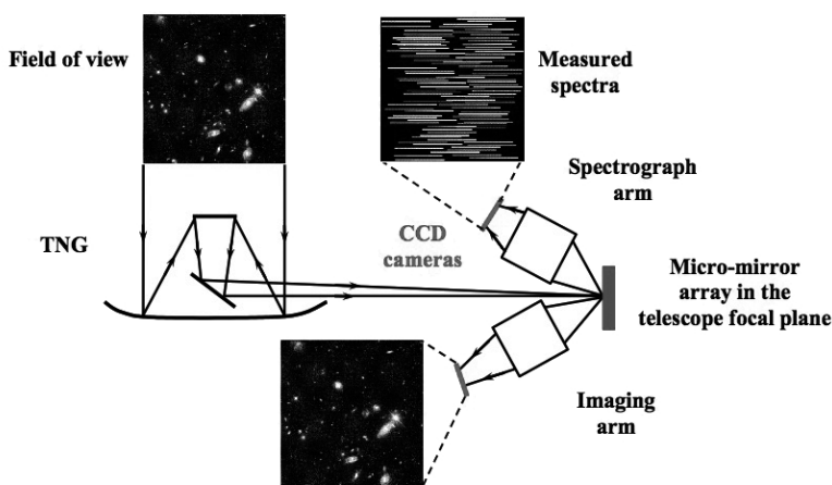
Figure 1. Principle of BATMAN spectro-imager
