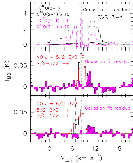
Figure 8. Upper panel: Residual of the C^{18}O(2-1) and C^{17}O(2-1) emission after Gaussian fit, showing the outflow wings. The vertical dashed line indicates the ambient LSR velocity ( +8.6 \text{ km s}^{-1} , Chen et al. 2009). Middle and bottom panel: The purple filled histogram shows the residual after Gaussian fit (red) of the NO ^2\Pi_{1/2} J = 5/2 - 3/2 F_{ul} = 7/2 - 5/2 ; 5/2 - 3/2 , and 3/2 - 1/2 ; p_{ul} = + \rightarrow - emission (black).
