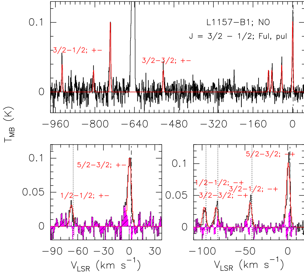
Figure 6. Upper panel: Emission due to the NO ^2\Pi_{1/2} J = 3/2 - 1/2 spectral pattern (black histogram; see Table 1; in T_{\text{mb}} scale after correction for beam dilution, see text) observed towards L1157-B1 with the IRAM 30-m antenna. The red line shows the best fit obtained with the GILDAS–Class package using the simultaneous fit of all the hyperfine components (see Table 2). For sake of clarity, the hyperfine components which are not indicated in the upper panel are labelled in the zoom-in in the lower panels. The spectrum is centred at the frequency of the hyperfine component F_{\text{ul}} = 5/2 - 3/2 ; p_{\text{ul}} = - \rightarrow + (150176.48 MHz). The vertical dashed line indicates the ambient LSR velocity ( +2.6 \text{ km s}^{-1} , Bachiller et al. 2001). Bottom-right panel: Zoom in of the Upper panel. Dotted lines points the hyperfine components falling in that portion of the spectrum. The purple filled histogram shows the residual after Gaussian fit (red) of the NO emission (black). Bottom-left panel: Zoom in of the Upper panel, after having centred the spectrum at the frequency of the hyperfine component F_{\text{ul}} = 5/2 - 3/2 ; p_{\text{ul}} = + \rightarrow - (150546.52 MHz).
