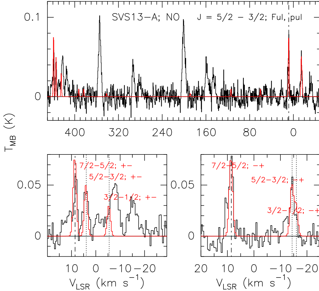
Figure 3. Upper panel: Emission due to the NO ^2\Pi_{1/2} J = 5/2 - 3/2 spectral pattern (black histogram; see Table 1; in T_{\text{mb}} scale after correction for beam dilution, see text) observed towards SVS13-A with the IRAM 30-m antenna. The red line shows the best fit obtained with the GILDAS-Class package using the simultaneous fit of all the hyperfine components (see Table 2). For sake of clarity, the hyperfine components are not indicated in the upper panel are labelled in the zoom-in in the lower panels. The spectrum is centred at the frequency of the hyperfine component F_{\text{ul}} = 7/2 - 5/2 ; p_{\text{ul}} = + \rightarrow - (250436.85 MHz). The vertical dashed line indicates the ambient LSR velocity ( +8.6 \text{ km s}^{-1} , Chen et al. 2009). Bottom-right panel: Zoom in of the Upper panel. Dotted lines indicate the hyperfine components falling in that portion of the spectrum. Note that the F_{\text{ul}} = 3/2 - 1/2 p_{\text{ul}} = - \rightarrow + line is blended with the brighter F_{\text{ul}} = 5/2 - 1/2 p_{\text{ul}} = - \rightarrow + one. The analysis of the residual is shown in Fig. 8. Bottom-left panel: Zoom in of the Upper panel, after having centred the spectrum at the frequency of the hyperfine component F_{\text{ul}} = 7/2 - 5/2 ; p_{\text{ul}} = + \rightarrow - (250796.44 MHz). The F_{\text{ul}} = 3/2 - 1/2 p_{\text{ul}} = + \rightarrow - line is blended with the 13_{9,4}-12_{9,3} intense emission at 250450.21 MHz due to \text{CH}_3\text{CHO-E} , a well known tracer of hot-corinos (as that around SVS13-A). For the legibility of the figure, given the complexity of this portion of the spectrum, the residual is not reported.
