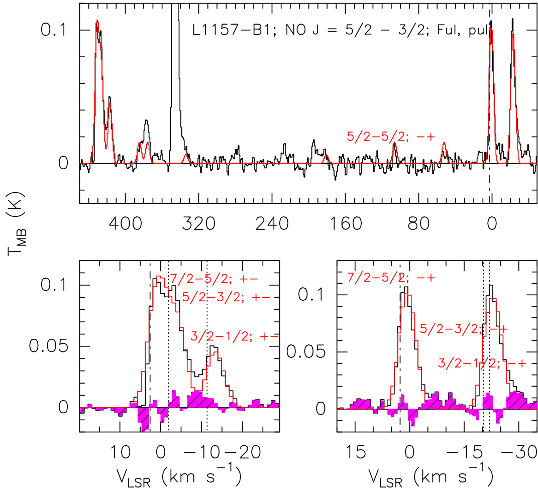
Figure 5. Upper panel: Emission due to the NO ^2\Pi_{1/2} J = 5/2 - 3/2 spectral pattern (black histogram; see Table 1; in T_{\text{mb}} scale observed towards L1157-B1 with the IRAM 30-m antenna. The red line shows the best fit obtained with the GILDAS-Class package using the simultaneous fit of all the hyperfine components (see Table 2). For sake of clarity, the hyperfine components which are not indicated in the upper panel are labelled in the zoom-in in the lower panels. The spectrum is centred at the frequency of the hyperfine component F_{\text{ul}} = 7/2 - 5/2 ; p_{\text{ul}} = + \rightarrow - (250436.85 MHz). The vertical dashed line indicates the ambient LSR velocity ( +2.6 \text{ km s}^{-1} , Bachiller et al. 2001). Bottom-right panel: Zoom in of the Upper panel. Dotted lines indicate the hyperfine components falling in that portion of the spectrum. Note that the F_{\text{ul}} = 3/2 - 1/2 p_{\text{ul}} = - \rightarrow + line is blended with the brighter F_{\text{ul}} = 5/2 - 1/2 p_{\text{ul}} = - \rightarrow + one. The purple filled histogram shows the residual after Gaussian fit (red) of the NO emission (black). Bottom-left panel: Zoom in of the Upper panel, after having centred the spectrum at the frequency of the hyperfine component F_{\text{ul}} = 7/2 - 5/2 ; p_{\text{ul}} = + \rightarrow - (250796.44 MHz).
