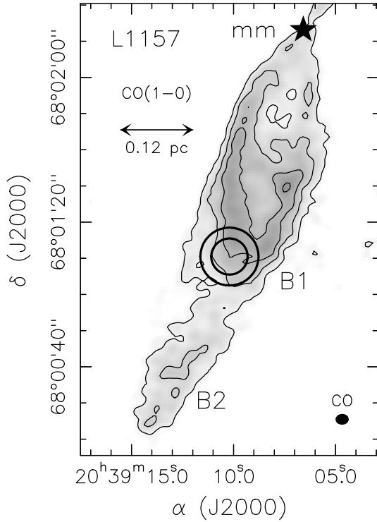
Figure 2. The L1157 southern blueshifted outflow as traced by CO(1-0) emission observed using the IRAM PdB interferometer (Gueth et al. 1996). The B1 and B2 cavities are labelled. The solid rings show the HPBW of the IRAM 30-m for the NO transitions detected at 2mm and 1mm towards B1 (see text). The star marks the position of the L1157-mm protostar.
