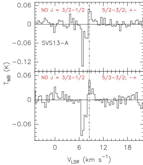
Figure 4. Upper panel: Spectral signatures due to the NO ^2\Pi_{1/2} J = 3/2 - 1/2 spectral pattern (black histogram; see Table 1; in T_{mb} scale after correction for beam dilution, see text) observed towards SVS13-A with the IRAM 30-m antenna. The spectrum is centred at the frequency of the hyperfine component F_{ul} = 5/2 - 3/2 ; p_{ul} = + \rightarrow - (150546.52 MHz). The vertical dashed line indicates the ambient LSR velocity (+8.6 km s ^{-1} , Chen et al. 2009). The absorption is due to emission in the OFF position, observed in wobbler mode with a throw of 180'' (see Sect. 3). Bottom panel: Same as for the Upper panel for the hyperfine component F_{ul} = 5/2 - 3/2 ; p_{ul} = - \rightarrow + (150176.48 MHz).
