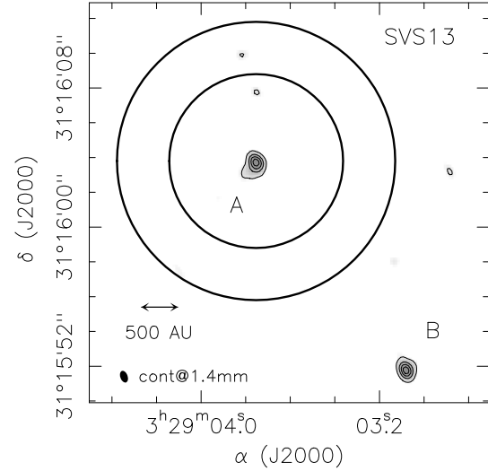
Figure 1. The SVS13 star forming cluster as observed using continuum emission at 1.4mm with the PdBI by De Simone et al. (2017). Two objects dominate at mm-wavelengths: the Class I system called A and the earlier Class 0 object called B. The solid rings show the HPBWs of the IRAM 30-m for the NO transitions detected at 2mm and 1mm towards SVS13-A.
