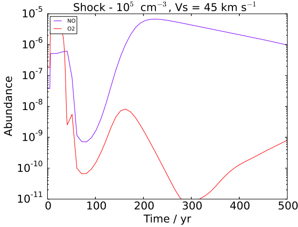
Figure 10. Phase 2 Theoretical fractional abundances of NO (blue) and O 2 (red) for our best matching shock model up to the dissipation length, with a pre-shock density of 10^5 \text{ cm}^{-3} and a shock velocity of 45 \text{ km s}^{-1} . The kinetic temperature of the pre-shock gas (Phase 1) is 10 K, while the post shock gas kinetic temperature is 80 K (Tafalla & Bachiller 1995)
