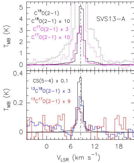
Figure 7. Emission detected towards SVS13-A with the IRAM 30-m in the 1mm spectral window with HPBW consistent with that used for the observations of NO ^2\Pi_{1/2} J = 5/2 - 3/2 . Upper panel: C^{18}O(2-1) and C^{17}O(2-1) lines (in T_{mb} scale; also increased by different factors to show the outflow wings; dotted histograms). The vertical dashed line indicates the ambient LSR velocity ( +8.6 \text{ km s}^{-1} , Chen et al. 2009). Bottom panel: ^{13}C^{18}O(2-1) , ^{13}C^{17}O(2-1) , and CS(5-4) profiles, scaled to be drawn on the same scale.
