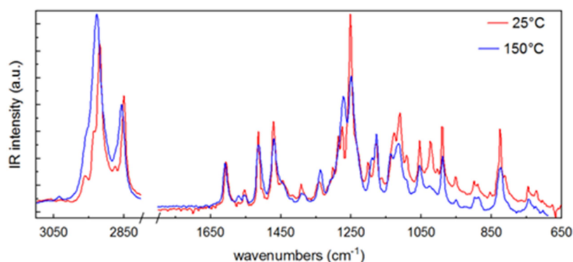
Figure 6 – FT-IR of a DTE-7 in the solid state at 25°C (red) and in the melt state at 150°C (blue).
