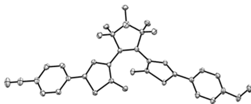
Figure S3. ORTEP representation of the molecular structures for the five novel DTE structures reported in this work.
