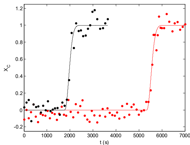
Figure 9 - Evolution of the crystallization fraction of DTE-7 obtained from the FT-IR normalized area of the 1023 cm -1 band for isothermal crystallization at 60°C (black dots) and 65°C (red dots). The solid line represents the Avrami fitting at each temperature.
