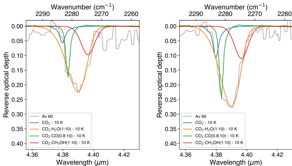
Extended Data Figure 4. Observed absorption profile of the 13 CO 2 asymmetric stretching, around 4.39 \mu\text{m} , in NIR38 (left panel) and J110621 (right panel). To demonstrate the ice chemical environment that best reproduces the observed feature peak, the colored curves show the scaled profiles of 13 CO 2 in laboratory spectra of the following ice mixtures at 10 K: pure CO 2 (blue), H 2 O:CO 2 (orange), CO 2 :CO (green), and CO 2 :CH 3 OH (red). In all the ice mixtures, CO 2 is diluted in a ratio of \sim 1:10 , with 12 CO 2 / 13 CO 2 \sim 90 .
