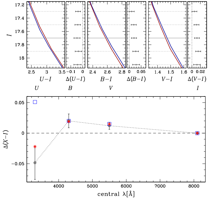
Fig. 15. Top panels: MS fiducial in 3 X - I CMDs ( X = U, B, V ) of NGC 6121. The horizontal lines represent the magnitudes I_{\text{CUT}} for which the color distance between the two MSs is calculated. For each I_{\text{CUT}} the error in \Delta(X - I) is shown. Bottom panel: X - I color distance between rMS and bMS at I_{\text{CUT}} = 17.7 as a function of the central wavelength of the X filter. Observations are represented with gray dots. Red asterisks are the best-fitting model, while blue squares are the results obtained calculating synthetic colors of two MS stars with the same light-element chemical composition, but different He content. The blue squares demonstrate that the abundance of light elements assumed in the model does not affect the results of the He abundance of the two MSs in the optical colors, but strongly affects the U band.
