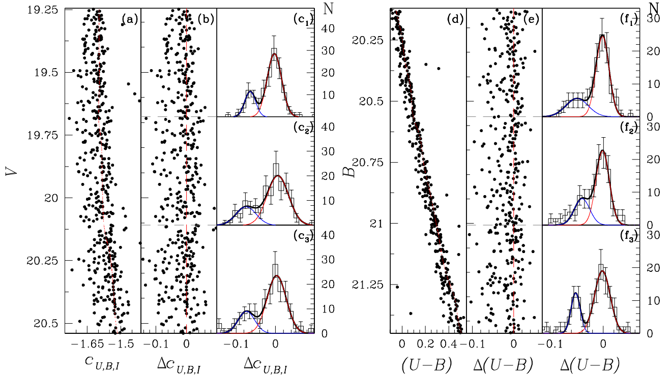
Fig. 10. Procedure to estimate the fraction of rMS and bMS stars in NGC 6752 using the V versus c_{U,B,I} diagram (panels a , b ), and the B versus U - B CMD (panels d , e ), and f ). Panels a and d ) reproduce the same diagrams as Figs. 8 and 5. The red line is the rMS fiducial line. Panels b ) and e ) show the verticalized MS. The histogram distribution of \Delta(\text{color}) for the stars of the panel b ) and e ) is plotted in panels c ) and f ) for three intervals of magnitude. The thick black lines, superimposed to each histogram, are the best-fitting biGaussian functions, whose components are colored red and blue. In the case of V versus c_{U,B,I} CMD, we found that rMS and bMS contain 77 \pm 4\% and 23 \pm 8\% of MS stars in panel c1 ), 74 \pm 5\% and 26 \pm 8\% of MS stars in panel c2 ) and, 75 \pm 5\% and 25 \pm 8\% of the MS stars, respectively. In the case of B versus (U - B) CMD, we found that rMS and bMS contain 72 \pm 5\% and 28 \pm 8\% of MS stars in panel f1 ), 74 \pm 6\% and 26 \pm 9\% of MS stars in panel f2 ), 73 \pm 5\% and 27 \pm 8\% of MS stars in panel f3 ), respectively.
