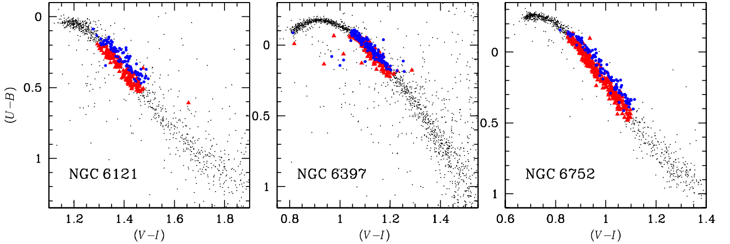
Fig. 7. Color-color diagrams for NGC 6121 ( left panel ), NGC 6397 ( central panel ), and NGC 6752 ( right panel ). In red (triangles) and blue (dots) we show the rMS and bMS as defined in Fig. 6
