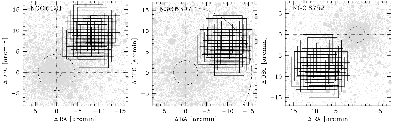
Fig. 1. Dither pattern of the FORS2 images taken in the fields of NGC 6121 ( left ), NGC 6397 ( middle ), and NGC 6752 ( right ). The dotted, dashed, and dashed-dotted circles indicate the core, half-light, and tidal radius of the three GCs. NGC 6397 and NGC 6752 are both post-core-collapse clusters.
