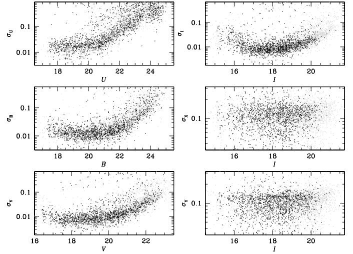
Fig. 2. Photometric ( left panels and top right panel ) and position residuals ( middle and bottom right panels ) from single measurements in the single images of NGC 6121 plotted as a function of the average magnitude. Gray points show all detected stars; black points refer to proper motion selected stars. In the case of NGC 6752 and NGC 6397, the distributions are similar.
