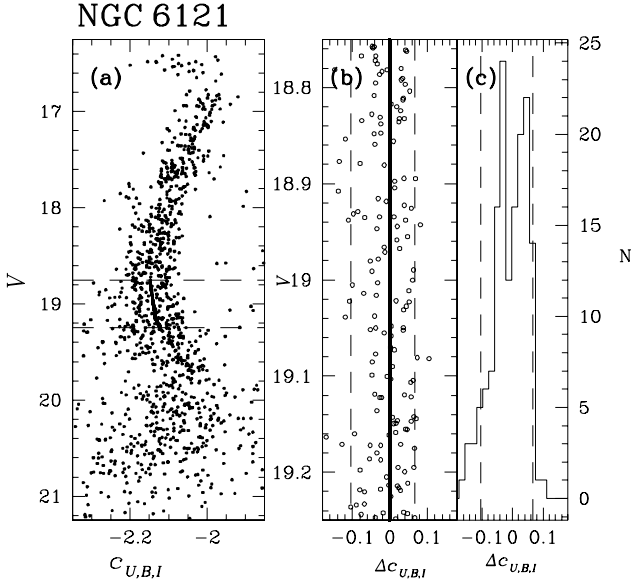
Fig. 9. Procedure to estimate the MS width for NGC 6121. Panel (a) shows the V versus c_{U,B,I} CMD of NGC 6121. The thick line is the MS fiducial line (see text for details). Panel (b) shows the verticalized MS between the two dashed lines of panel (a). Panel (c) is the distribution of the color for the stars of panel (b).
