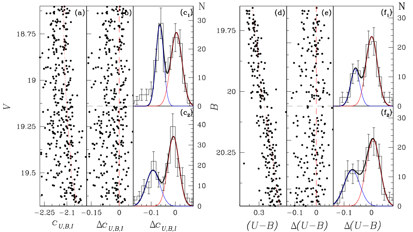
Fig. 11. As in Fig. 10, in the case of NGC 6121. In the case of V versus c_{U,B,I} CMD, we found that rMS and bMS contain 60 \pm 7\% and 40 \pm 8\% of MS stars in panel c1 ), 61 \pm 6\% and 39 \pm 7\% of MS stars in panel c2 ), respectively. In the case of B versus (U - B) CMD, we found that rMS and bMS contain 67 \pm 7\% and 33 \pm 10\% of MS stars in panel f1 ), 75 \pm 13\% and 25 \pm 14\% of MS stars in panel f2 ), respectively.
