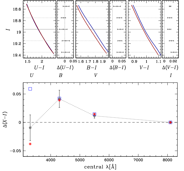
Fig. 16. As in Fig. 15, in the case of NGC 6752. In the top panels , the fiducial blue is that of the MSa and the red fiducial is for MSbc.
