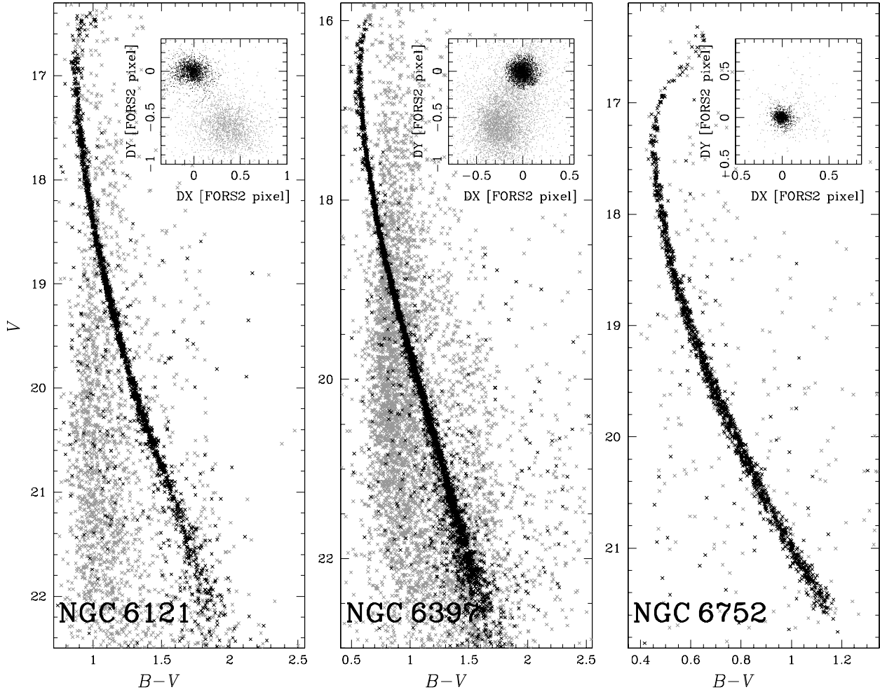
Fig. 4. The V versus B - V CMD of stars in the field of view of NGC 6121 ( left ), NGC 6397 ( middle ), and NGC 6752 ( right ). The insets show the vector-point diagram of stellar displacements along the X and Y direction. Black and gray points indicate stars that, according to their proper motions, are considered cluster members and field stars, respectively (see text for details).
