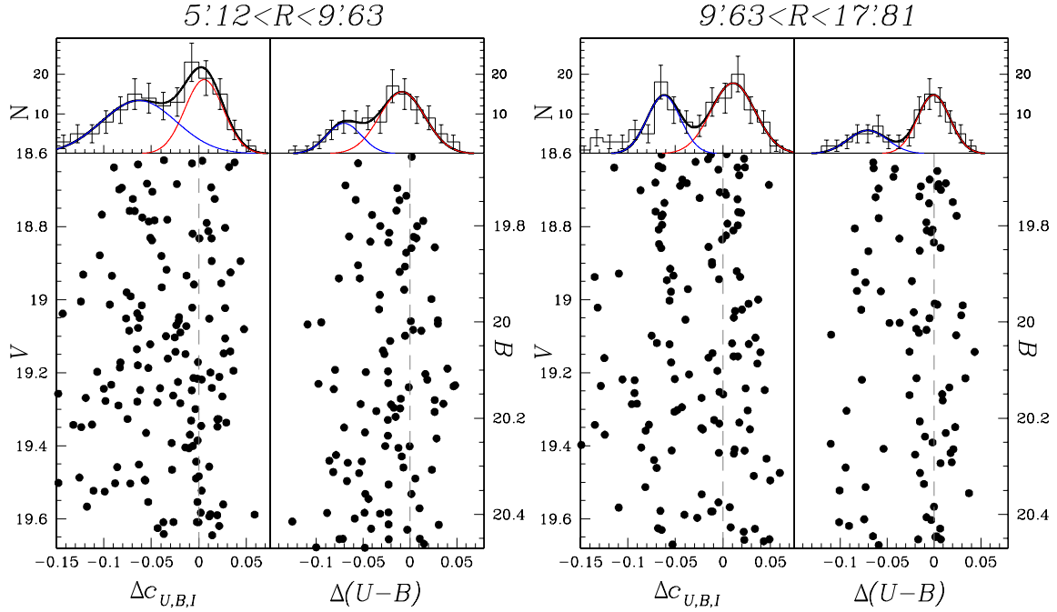
Fig. 14. Color distribution analysis for the MSs stars of NGC 6121 in two different radial bin, containing almost the same number (754 and 755) of stars. In the inner field ( left panels ) we found that rMS and bMS contain 42 \pm 20\% and 58 \pm 20\% of MS stars, respectively, in the V versus c_{U,B,I} CMD, and 73 \pm 16\% and 27 \pm 17\% of MS stars, respectively, in the B versus (U - B) CMD. In the outer field ( right panels ) we found that rMS and bMS contain 62 \pm 6\% and 38 \pm 7\% of MS stars, respectively, in the V versus c_{U,B,I} CMD, and 67 \pm 6\% and 33 \pm 9\% of MS stars, respectively, in the B versus (U - B) CMD.
