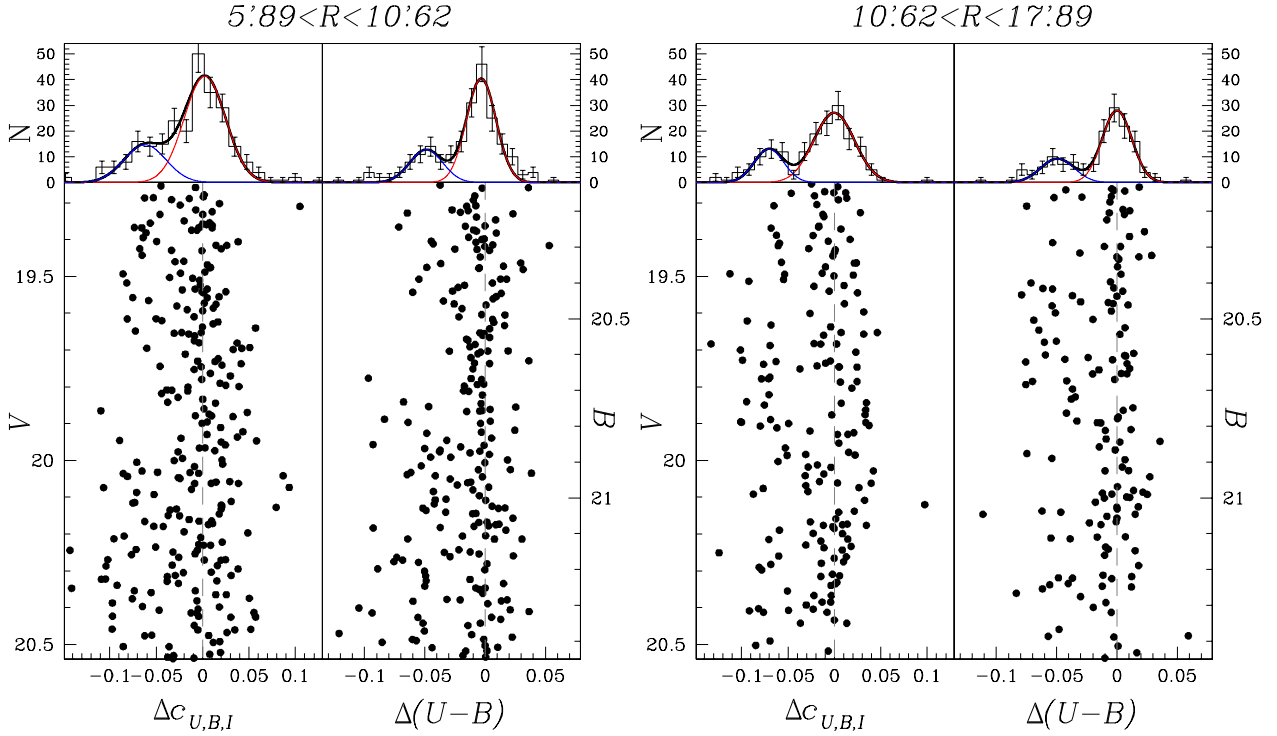
Fig. 12. Color distribution analysis for the MSs stars of NGC 6752 in two different radial bin, containing almost the same number (855 and 854) of stars. In the inner field ( left panels ) we found that MSa (blue) and MSbc (red) contain 28 \pm 6\% and 72 \pm 4\% of MS stars, respectively, in the V versus c_{U,B,I} CMD, and 27 \pm 6\% and 73 \pm 4\% of MS stars, respectively, in the B versus (U - B) CMD. In the outer field ( right panels ) we found that MSa and MSbc contain 26 \pm 7\% and 74 \pm 4\% of MS stars, respectively, in the V versus c_{U,B,I} CMD, and 29 \pm 8\% and 71 \pm 6\% of MS stars, respectively, in the B versus (U - B) CMD.
