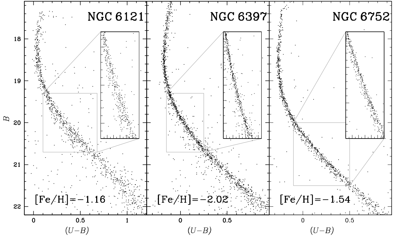
Fig. 5. The B versus (U - B) CMD for NGC 6121 (left), NGC 6397 (middle), and NGC 6752 (right). The inset is a zoom around the upper MS. The CMDs only show the cluster members and are corrected by zero-point variations and differential reddening
