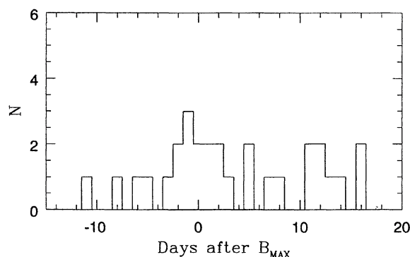
FIG. 4. Histogram showing the time with respect to B_{MAX} of the first photometric observation in B , V , or I . Note that for nearly one third of the SNe the photometric monitoring started before or at maximum light.
