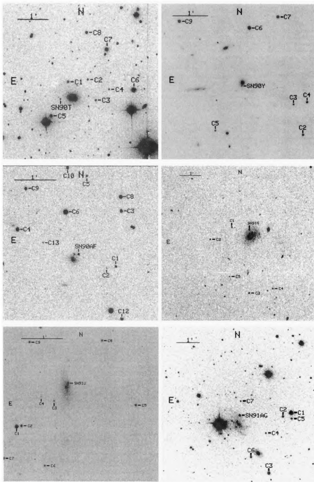
FIG. 1. V band CCD images of the 32 SNe Ia discovered in the course of the Calán/Tololo survey. The photometric sequence stars are labeled along with the SNe.
