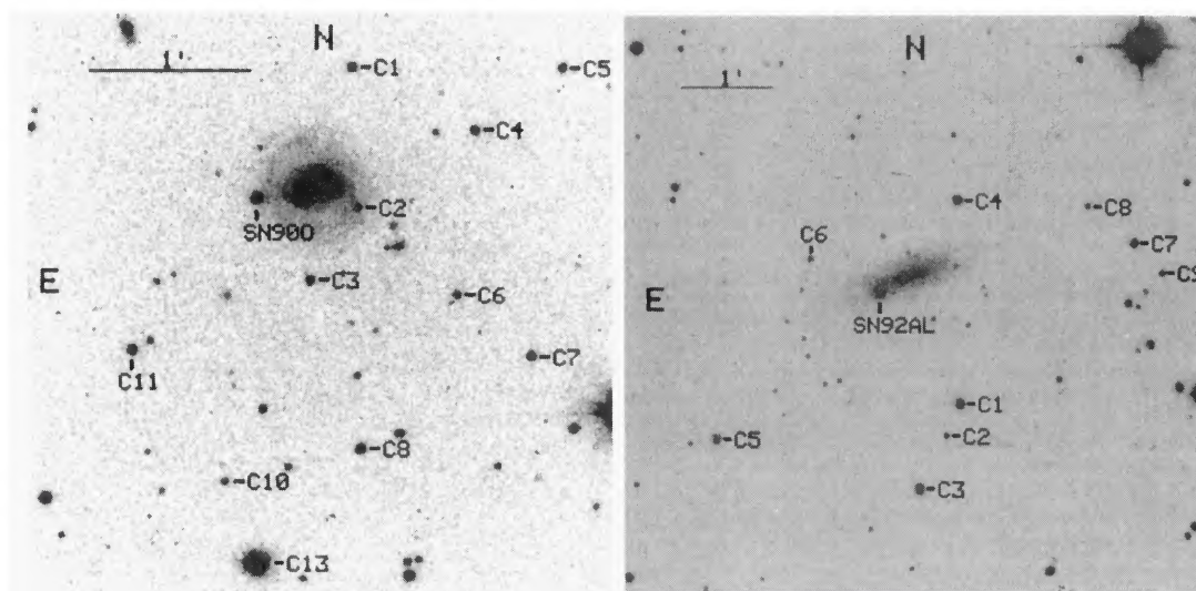
FIG. 2. V band CCD images of the two SNe Ia, 1990O and 1992al, discovered at other observatories and included in the Calán/Tololo follow-up photometric program. The photometric sequence stars are labeled along with the SNe.
