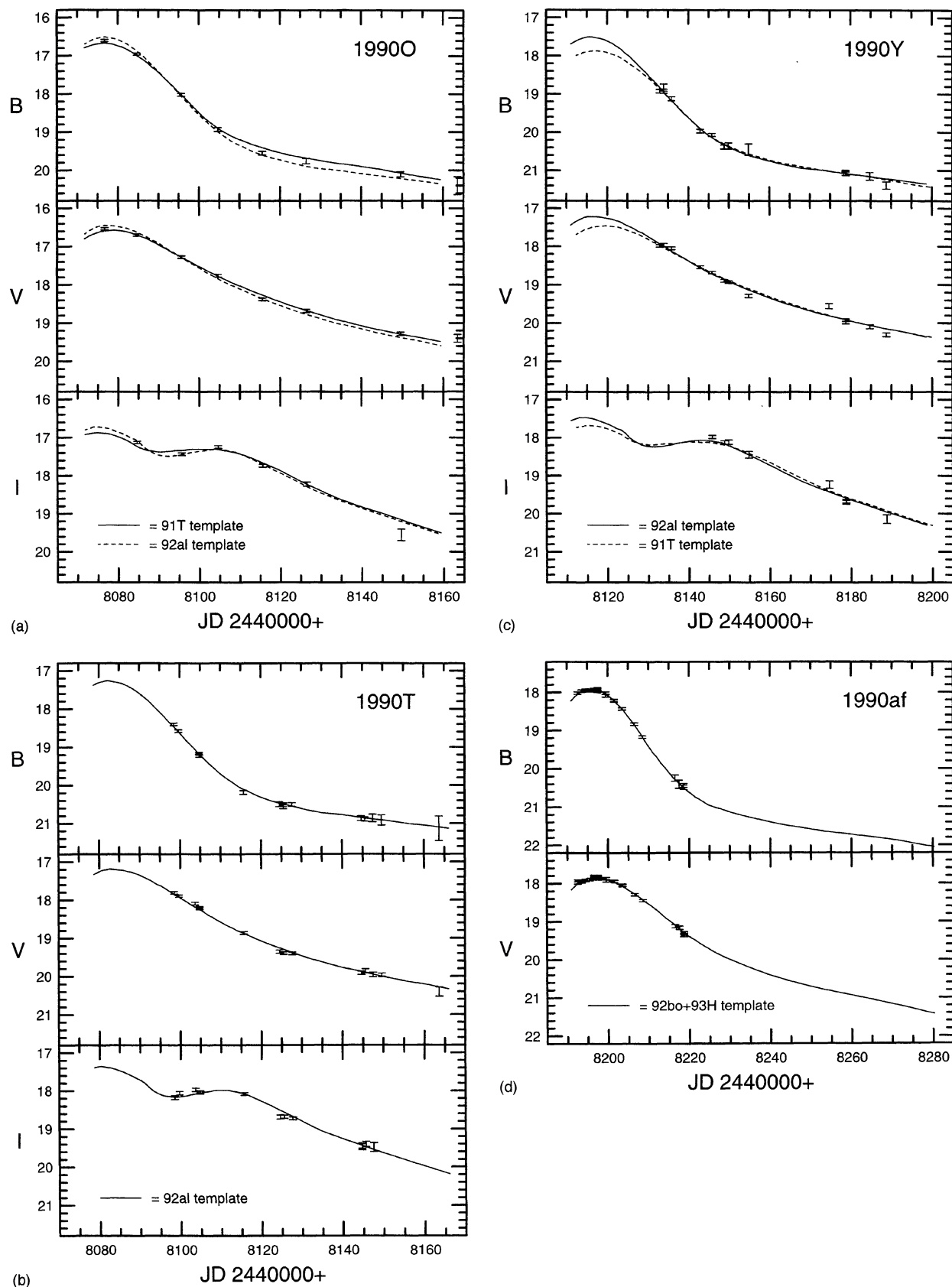
FIG. 3. B , V , and I light curves for the 29 SNe Ia. In all cases the solid lines correspond to the best-fitting template. The next-best fit is also shown as dashed lines when the difference in the reduced \chi^2 between the two best fits was \leq 1.5 .
