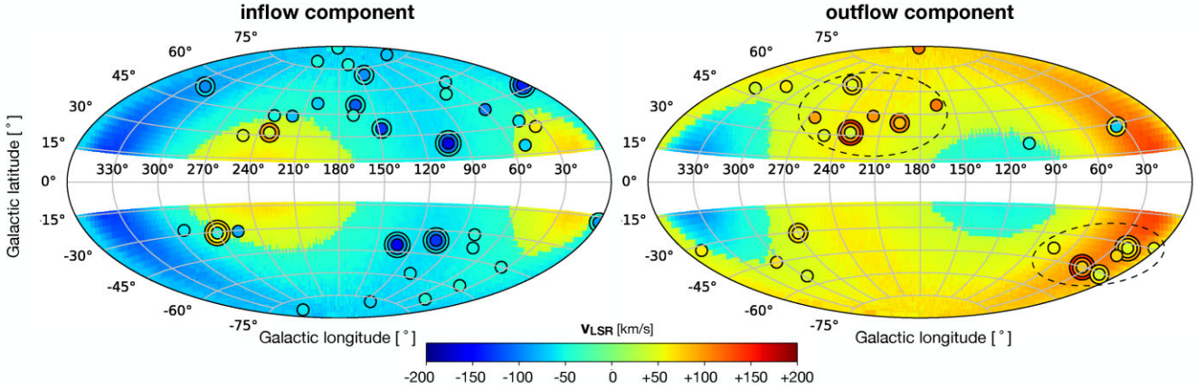
Figure 5. Comparison between the all-sky velocity fields predicted by our best-fitting inflow + outflow models (background colours) and the LSR velocity of the observed absorption features (coloured circles). Concentric circles are used when multiple detections are found towards the same target star. The map on the left-hand side (right-hand side) shows the 52 (33) absorbers compatible with the inflow (outflow) component. The dashed ellipses mark the locations of the biconic outflow encompassing most of the observed feature associated with the outflow component.
