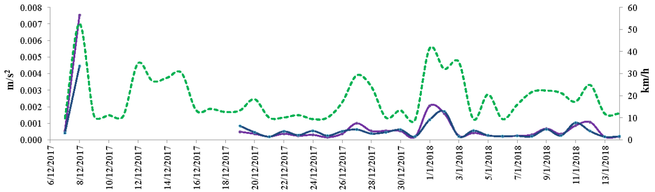
Figure 15. Daily average of the maximum hourly accelerations measured by S.2 vs. time along the x (blue) and y (red). directions. The dashed green line stands for the daily maximum wind speed.
